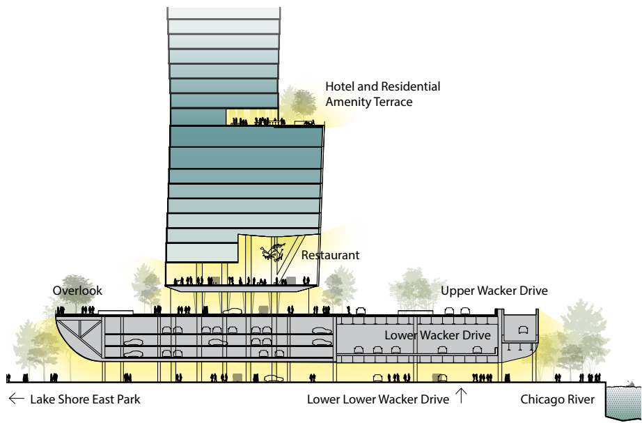
Figure 8. Resisting the fortress-like bases typical of many supertall towers, Vista enhances connections to the ground plane with new access points to Upper Wacker Drive, defining a generous connection between park and river. Additionally, publicly accessible spaces are distributed throughout the tower.
