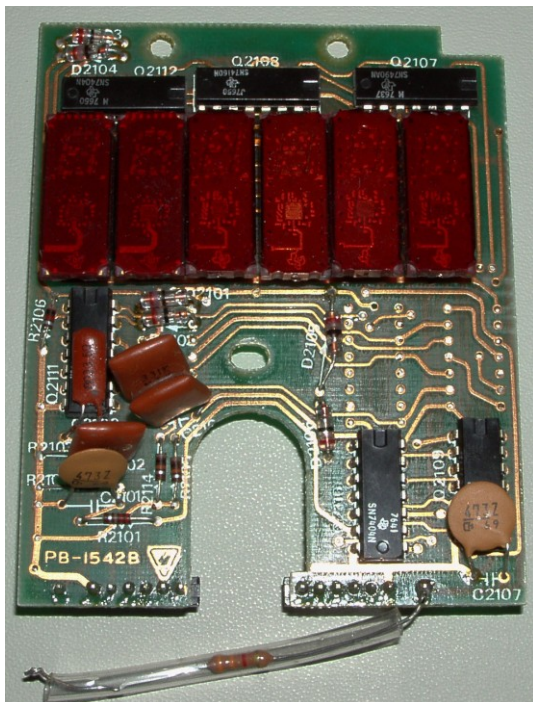
Figure 1 : PB-1542B Display Logic Unit
