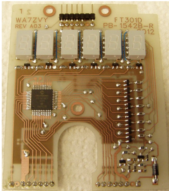
Figure 5: PB-1542B-R Display Logic Unit (top)
