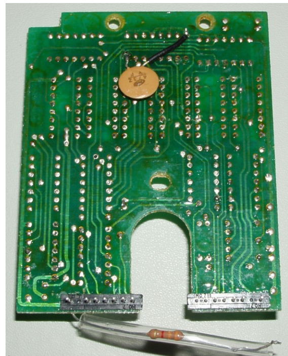
Figure 2 : PB1542B Display Logic Unit
