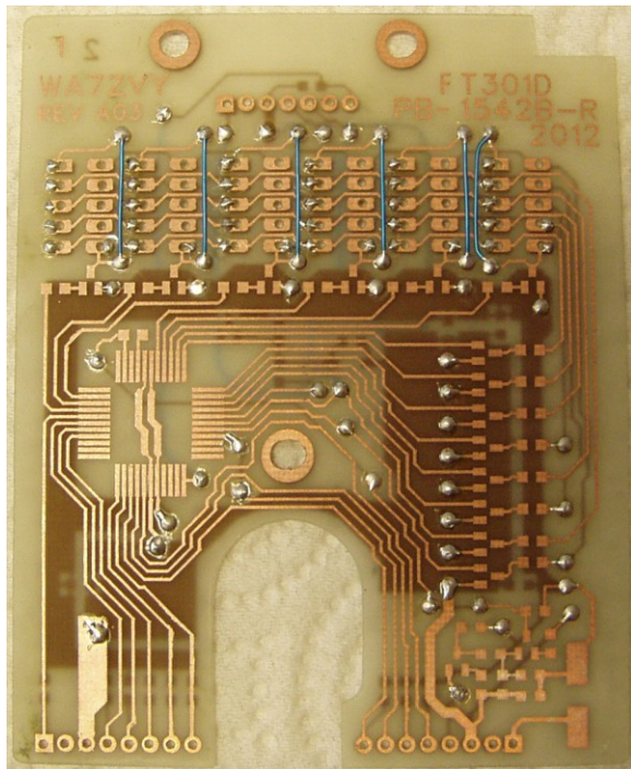
Figure 3: New Display Logic Unit PCB (top)
