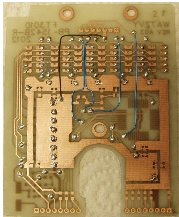
Figure 4: New Display Logic Unit PCB (bottom)
