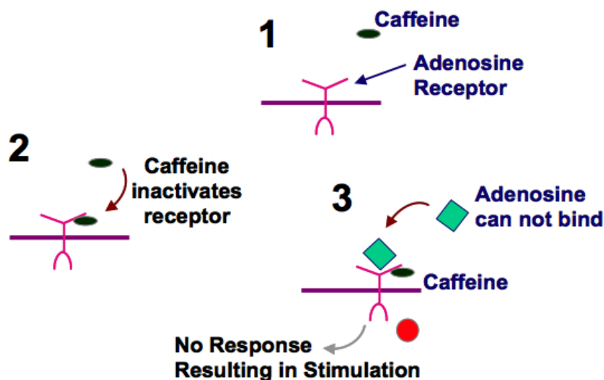
Figure 5.3 Mechanism of Action of Caffeine
