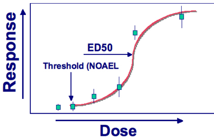
Figure 21.1 Dose Response
