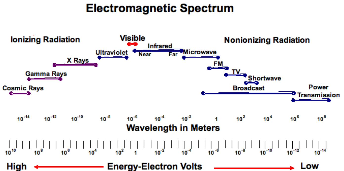
Figure 13.1 Electromagnetic Spectrum
