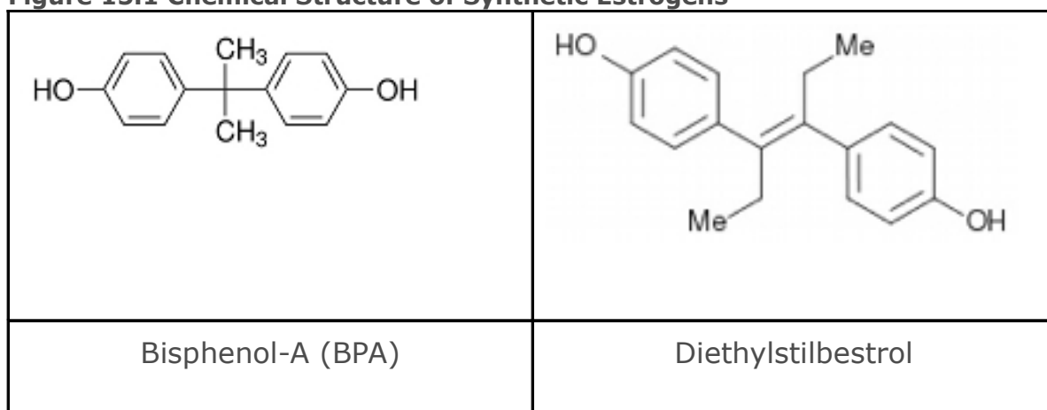
Figure 15.1 Chemical Structure of Synthetic Estrogens
