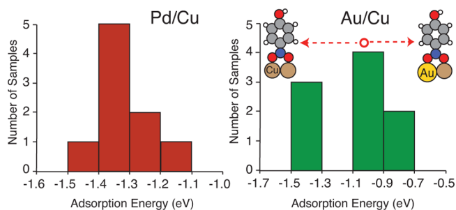
Figure 6. Histograms of the adsorption energies of PNP on nanoparticles of Pd/Cu and Au/Cu are shown. The y-axis of the histogram is the number of nanoparticles in the randomly generated sample of bimetallic alloys of the specified composition, and the x-axis is the binding energy of PNP. The Pd/Cu distribution is centered around a single ensemble average for binding energy; however, the Au/Cu binding energy has two peaks that correspond to the pure Cu site and the Au–Cu site.
