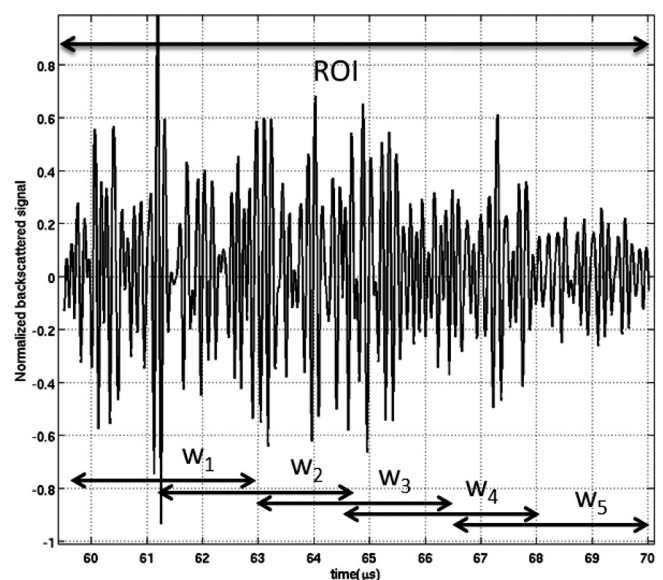
FIG. 2. Example of a backscattered RF signal from a ROI. This signal is gated by five overlapping windows (50% overlapping) denoted by w_1 , w_2 , w_3 , w_4 , and w_5 .
