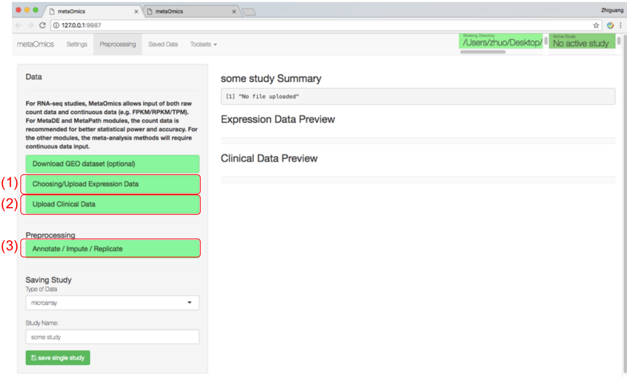
Figure 4: GUI for the preprocessing page
