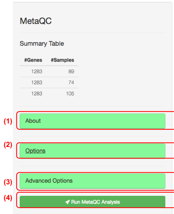
Figure 10: MetaQC options
