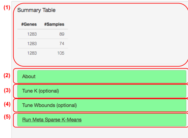
Figure 30: MetaClust homepage
