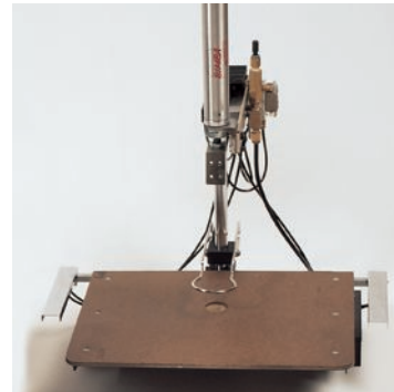
SPU6A01 Tablemount Hand Buttons Top Compression 1" Stroke
