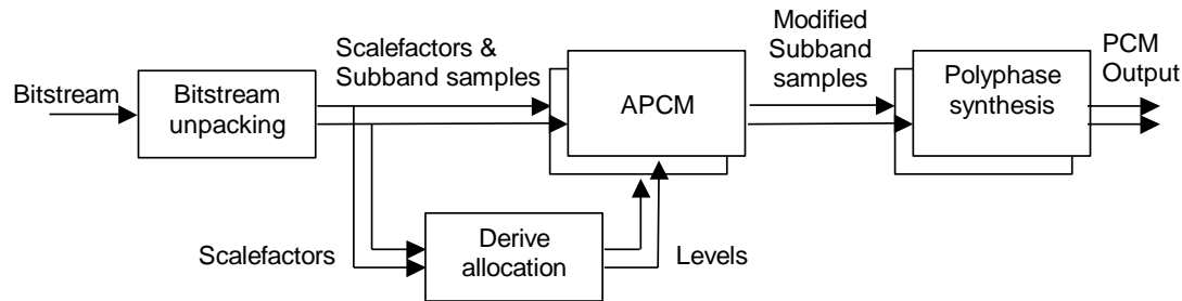
Figure 12.1: Diagram of the decoder
