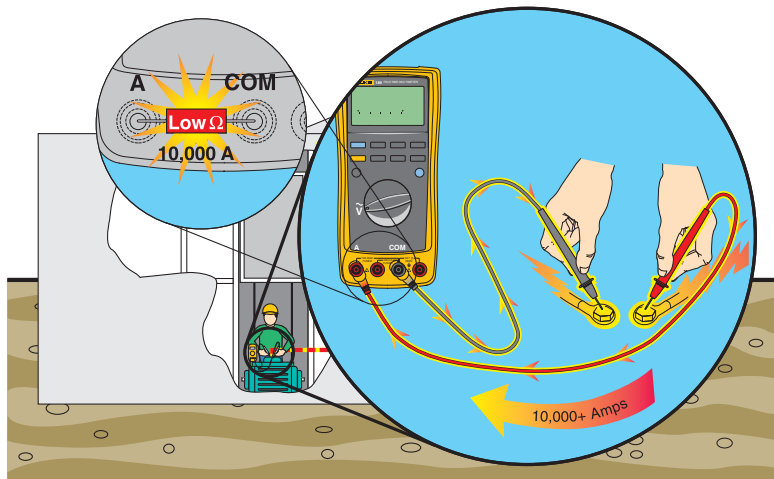
Figure 3. Misuse of DMM in Ammeter Mode.
