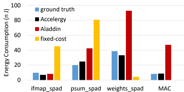
Figure 9: Energy breakdown within a single PE instance.
