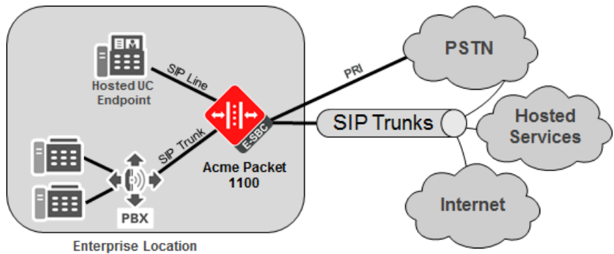
Figure 1. Acme Packet 1100 supports a wide range of deployment models and resiliency options, ensuring high service availability for small to medium sized business and remote office locations.
