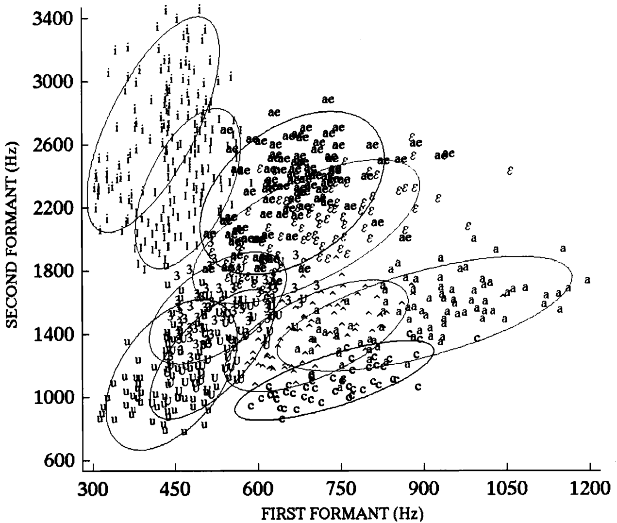
FIG. 4. Values of F_1 and F_2 for 46 men, 48 women, and 46 children for 10 vowels with ellipses fit to the data ("ae"= /æ/ , "a"= /ɑ/ , "c"= /ɔ/ , "λ"= /λ/ , "3"= /ɜ/ ). Measurements for /e/ and /o/ have been omitted, and the data have been thinned of redundant data points.
