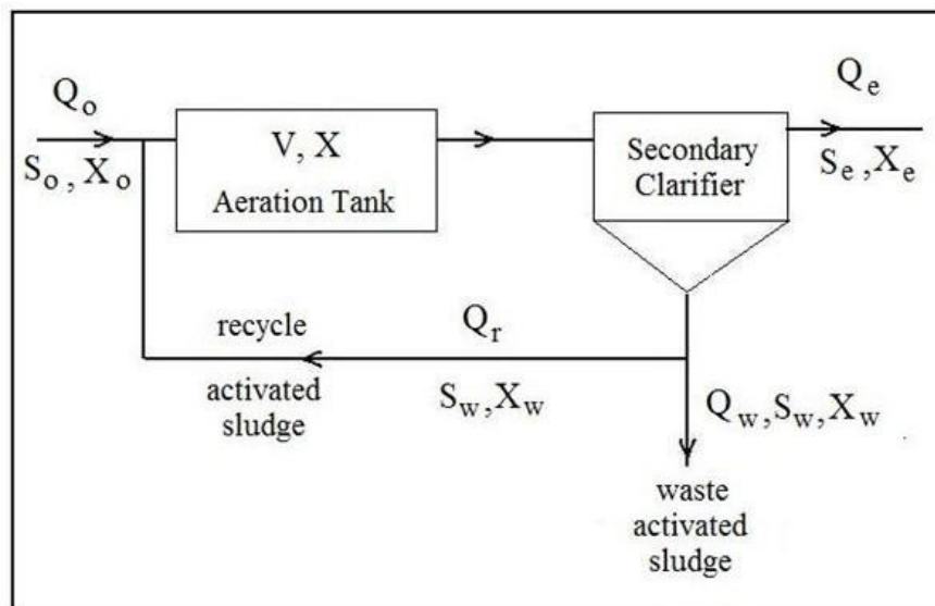
Activated Sludge Flow Diagram & Parameters
