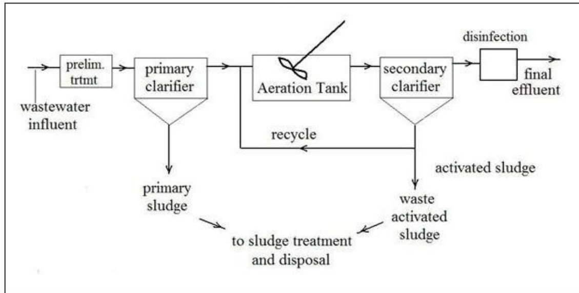
Completely Mixed Activated Sludge Flow Diagram
