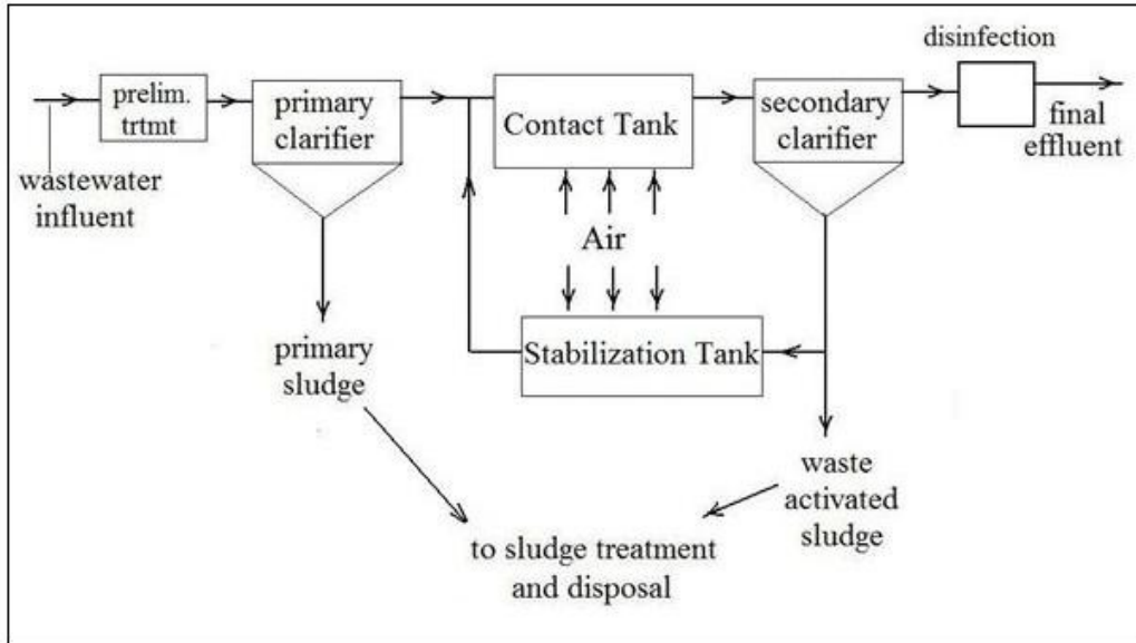
Contact Stabilization Activated Sludge Flow Diagram
