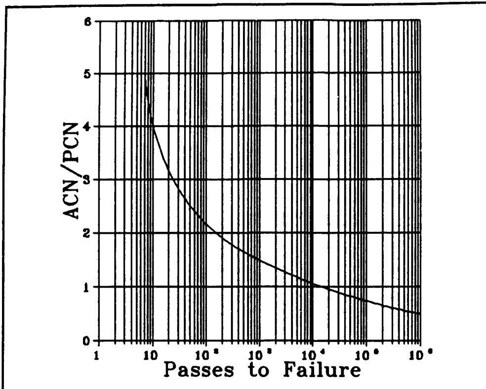
Figure D2. ACN/PCN versus allowable passes.
