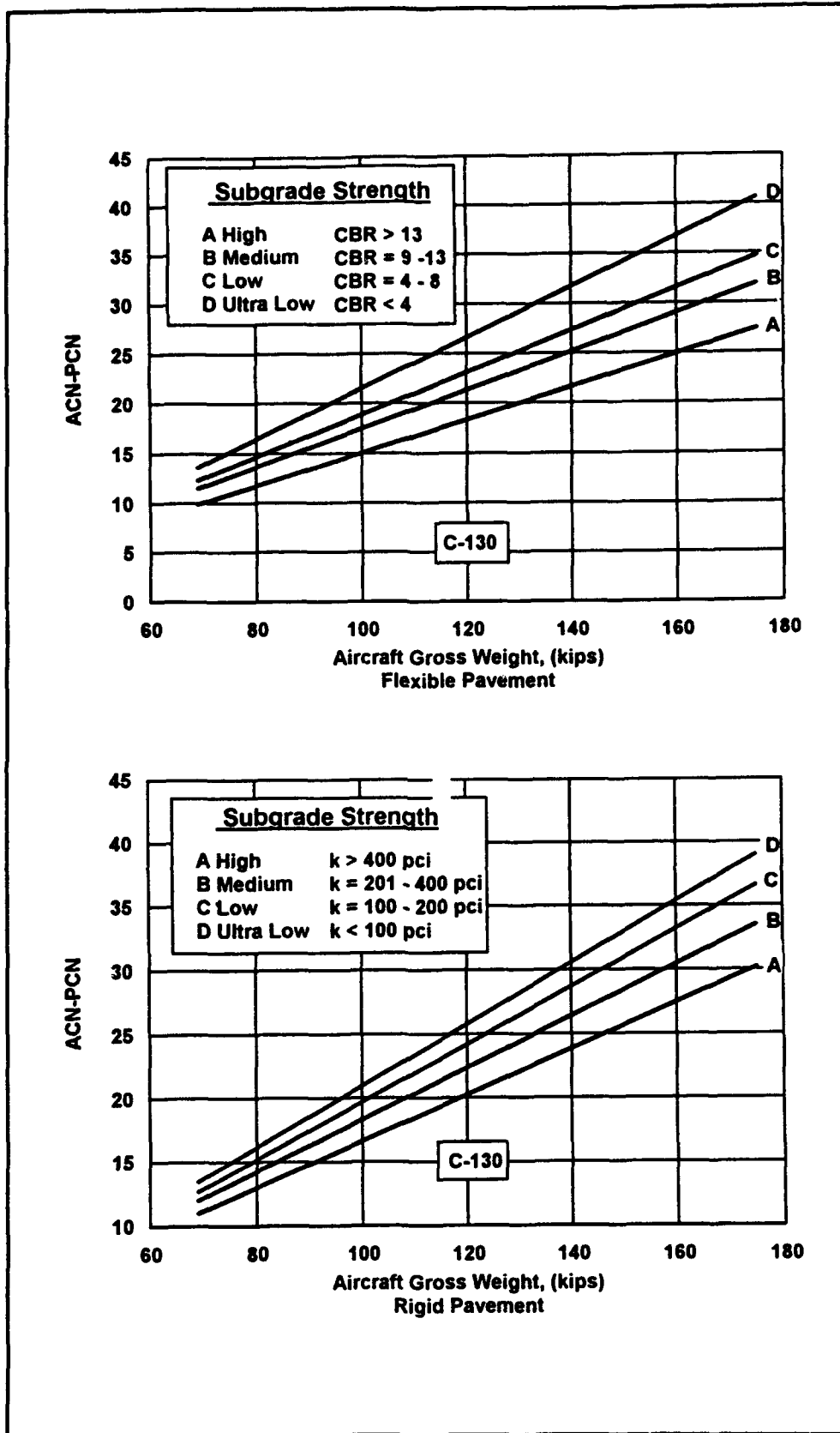
Figure D1. ACN curves for C-130 aircraft.
