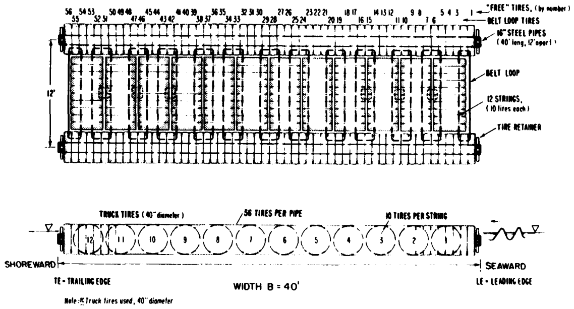
Figure 4. Schematic of PT-1 breakwater module.
