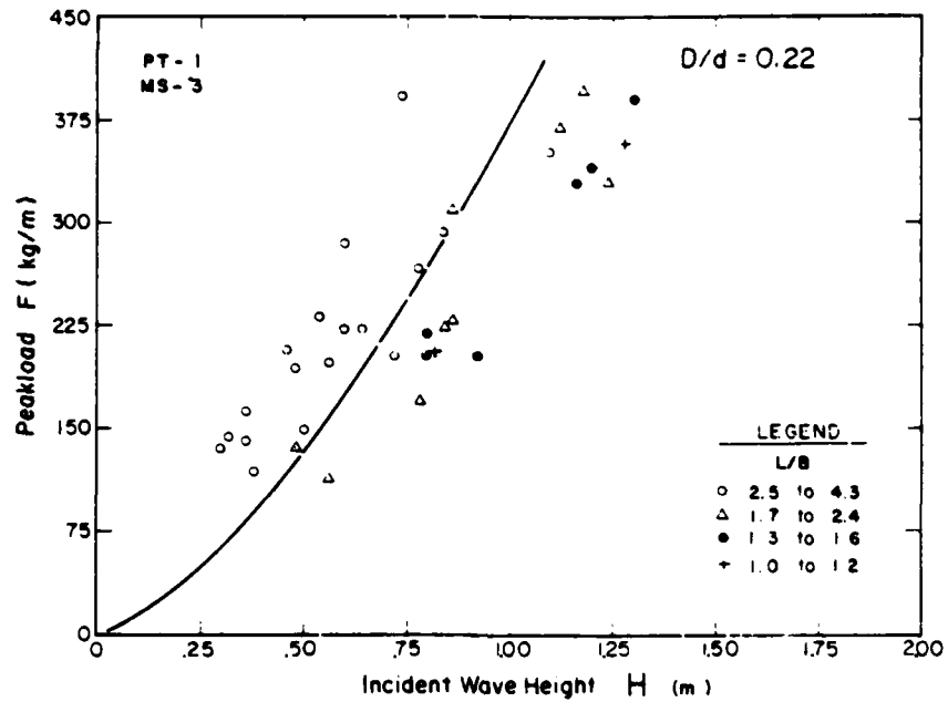
Figure 48. PT-1 peak mooring-force data (MS-3, d = 4.7 m).
