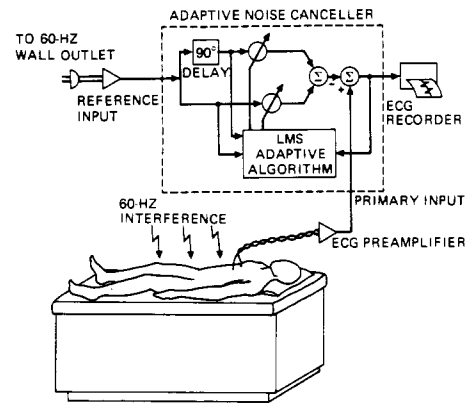
Fig. 10. Cancelling 60-Hz interference in electrocardiography.
