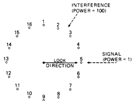
Fig. 20. Array configuration for adaptive sidelobe cancelling experiment.
