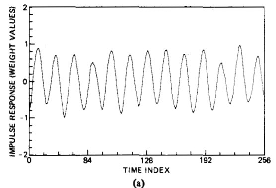
Fig. 25. Result of self-tuning filter experiment.
