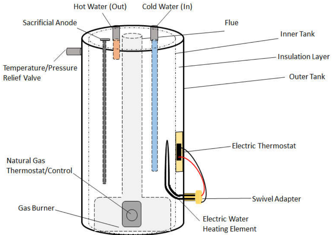
Figure 2: Natural gas tank with the Add-On Electric Water Heater and thermostat in place on side of tank.
