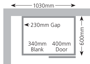
Full Height CB86FAFP Drawer Line CB86DAFP
