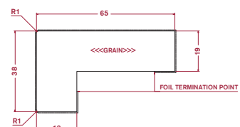
Square Universal Cornice and Pelmet CORPEL30F (Alta Gloss, Alta Matt, Minnesota, Plaza & Quadra only)
