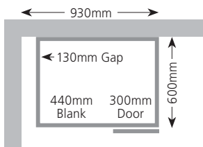
Full Height CB86FBFP Drawer Line CB86DBFP
