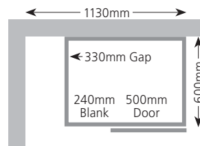
Full Height CB86FCFP Drawer Line CB86DCFP
