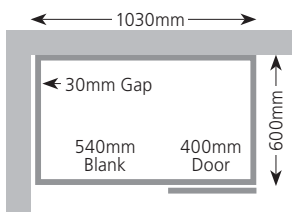
Full Height Door CB106FBFP Drawer Line CB106DBFP
