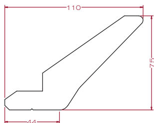
Tall Cornice CORCT30V (Austin and Oakham, only) CORCT30VPTO (Austin PTO, New England PTO and Wexford PTO only)
