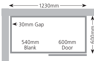
Full Height Door CB126FAFP Drawer Line CB126DAFP
