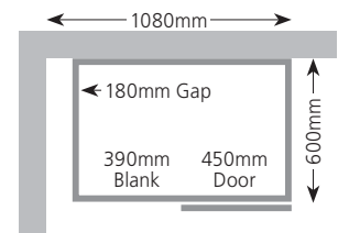
Full Height CB96FAFP Drawer Line CB96DAFP
