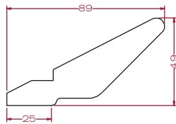
Modern Tangent Cornice CORT30P/CORT30V (Calgary, Cranbrook, Georgia, Newport & Rockfort only)
