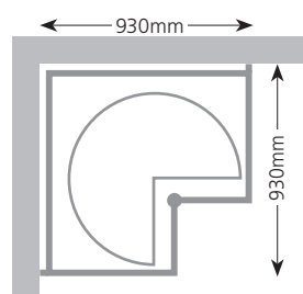
Full Height Door LCB99F Drawer Line LCB99D
