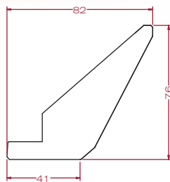
Square Foil Wrapped Pelmet UPST30V (Ashbourne only) UPST30PTO (Ashbourne PTO only)
