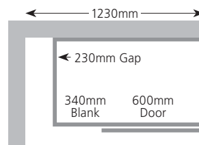
Full Height Door CB106FCFP Drawer Line CB106DCFP
