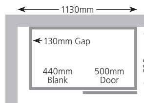
Full Height Door CB106FAFP Drawer Line CB106DAFP
