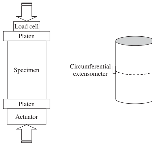
Figure 5-30 Circumferentially controlled test setup
