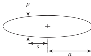
Figure 7-10 A crack under a pair of wedge forces on the left side
