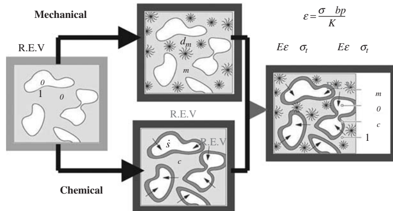
Figure 9-6 Conversion of chemical influence to mechanical effect
