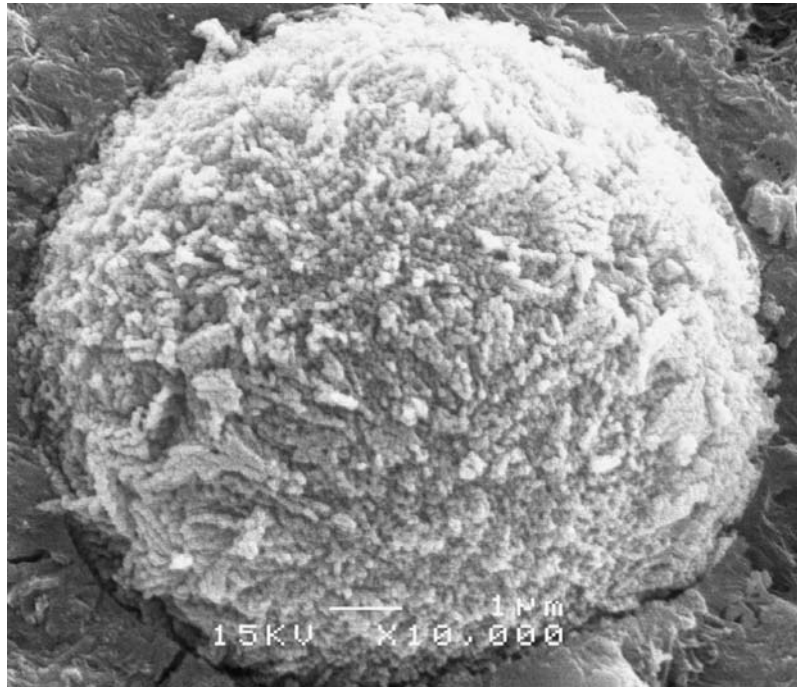
Figure 4-6 Reacted fly ash particle in concrete
