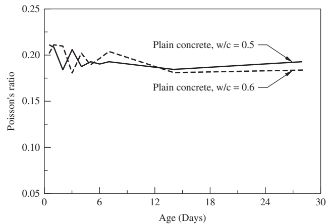
Figure 8-43 Poisson's ratio versus age
