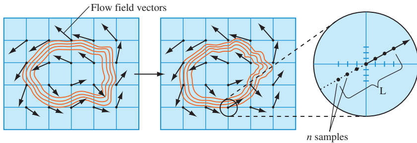
Figure 20.22 Line integral convolution with OpenGL.
