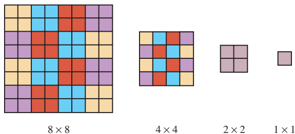
Figure 12.3 Recursive 2-way folding.
