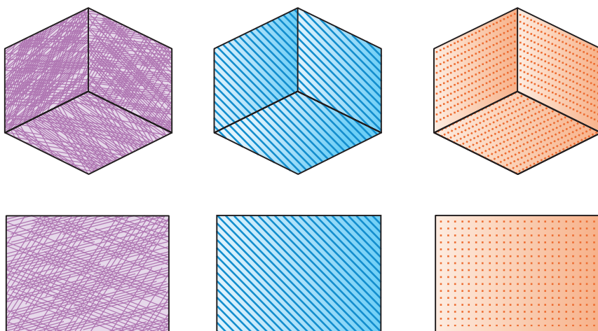
Figure 19.7 2D patterns.
