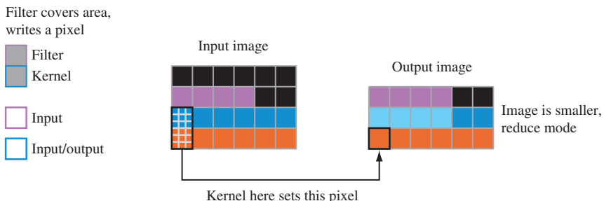
Figure 4.5 Convolution.
