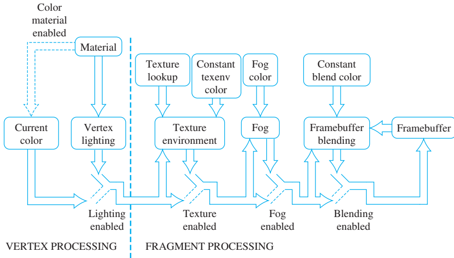
Figure 3.3 Color-processing path.
