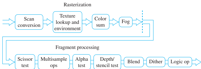
Figure 6.1 Rasterization pipeline.
