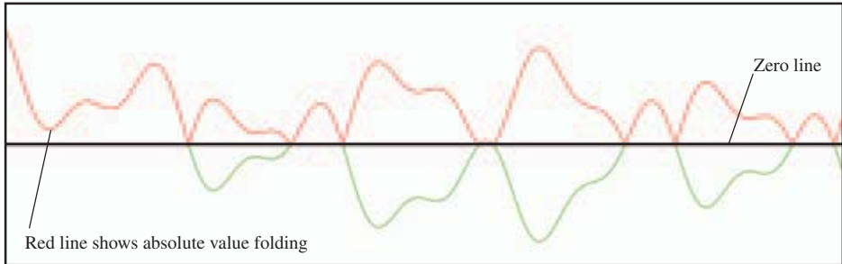
Figure 18.13 Turbulence.
