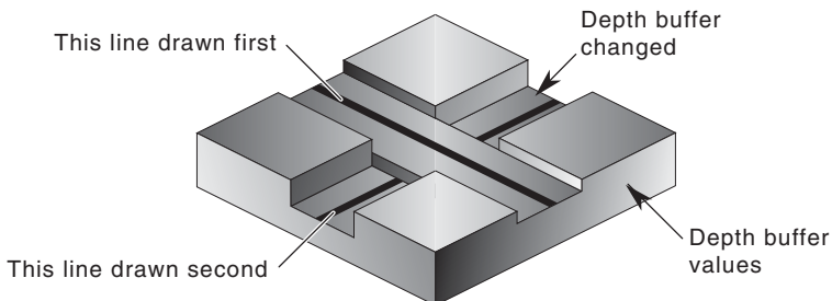
Figure 16.7 Haloed line.
