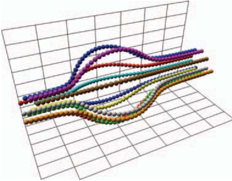
Figure 20.19 Particle tracing.
