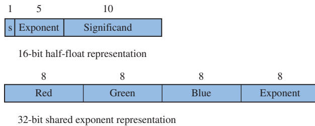
Figure 12.9 Half-float and RGBE HDR representations.
