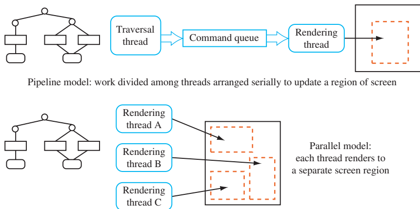
Figure 21.5 Multiple thread rendering models.
