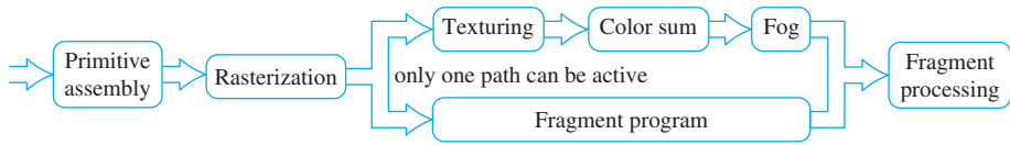
Figure 5.13 Fragment program functionality.
