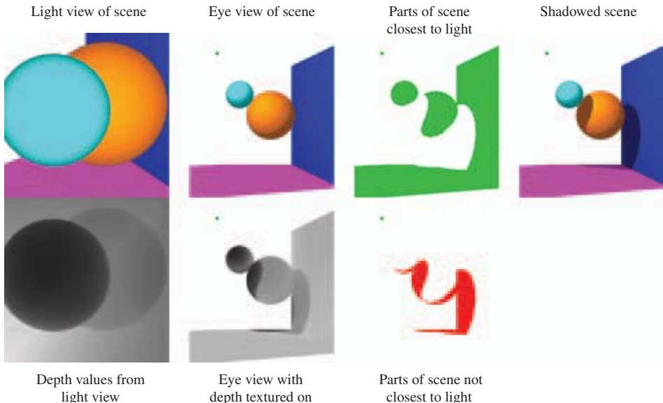
Figure 17.28 Shadow map.
