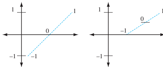
Figure 3.9 Biased representation.
