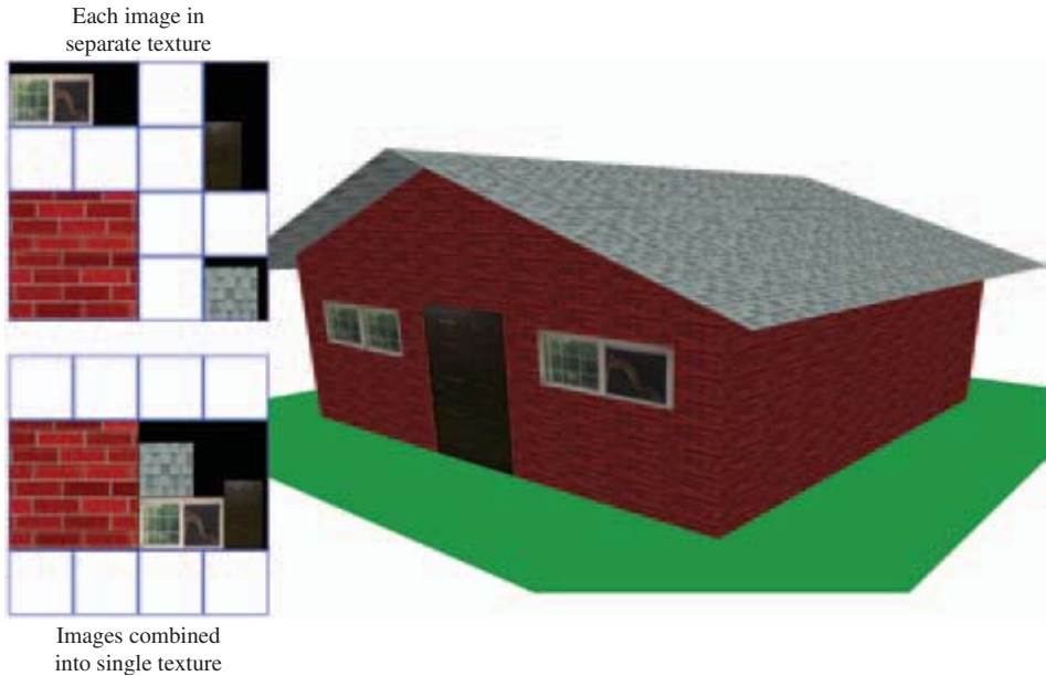
Figure 14.3 Texture mosaicing.
