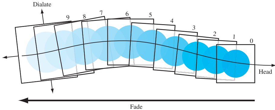
Figure 18.6 Vapor trail.
