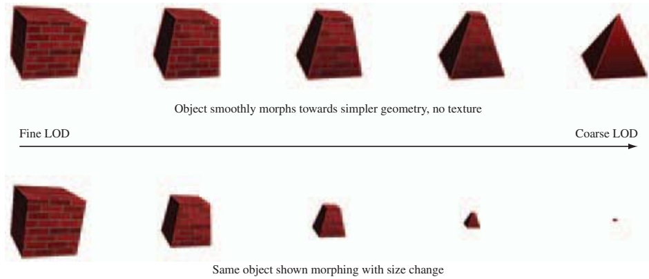
Figure 16.4 Morphing transition.
