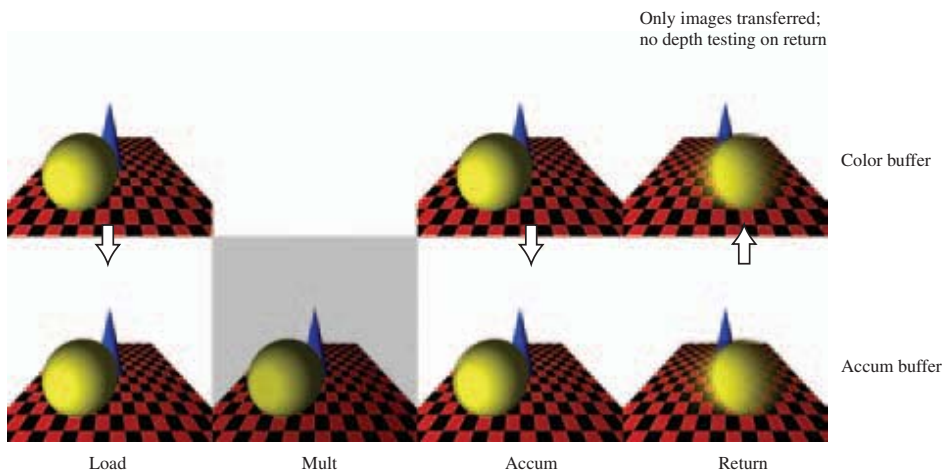
Figure 6.5 Accumulation buffer.
