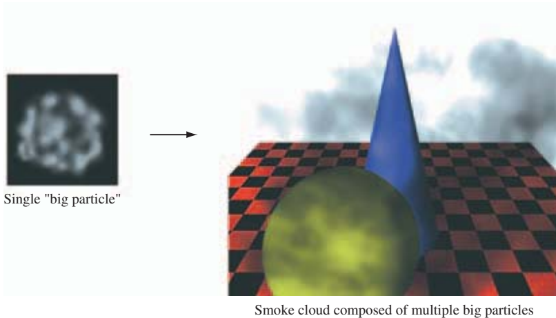
Figure 18.1 Big particles.
