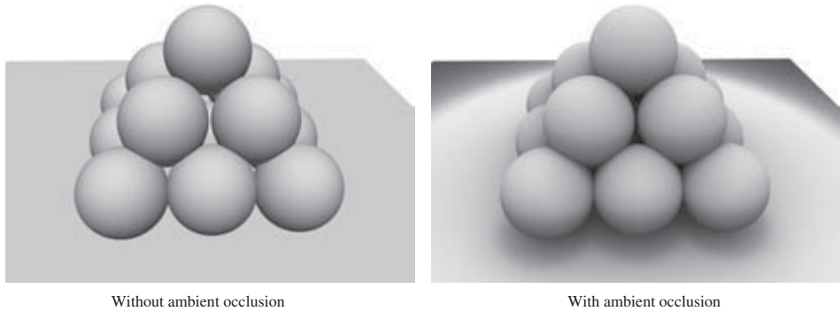
Figure 15.16 Ambient occlusion.
