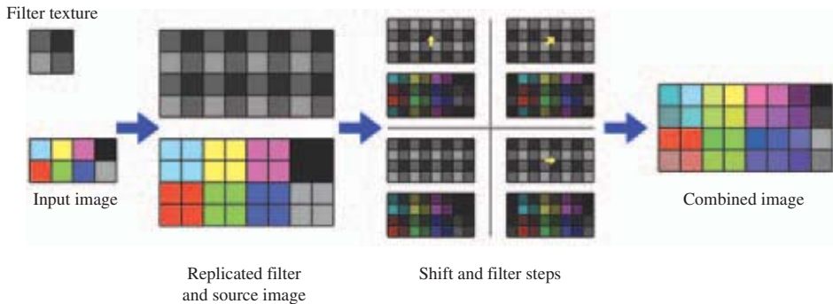
Figure 18.12 Output image.
