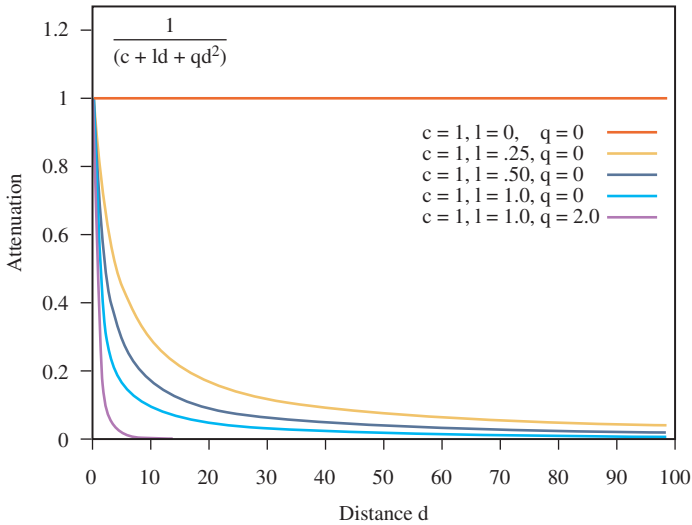
Figure 15.3 Attenuation function.
