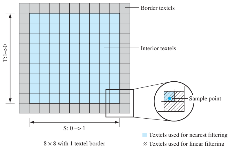
Figure 5.1 Texture borders.
