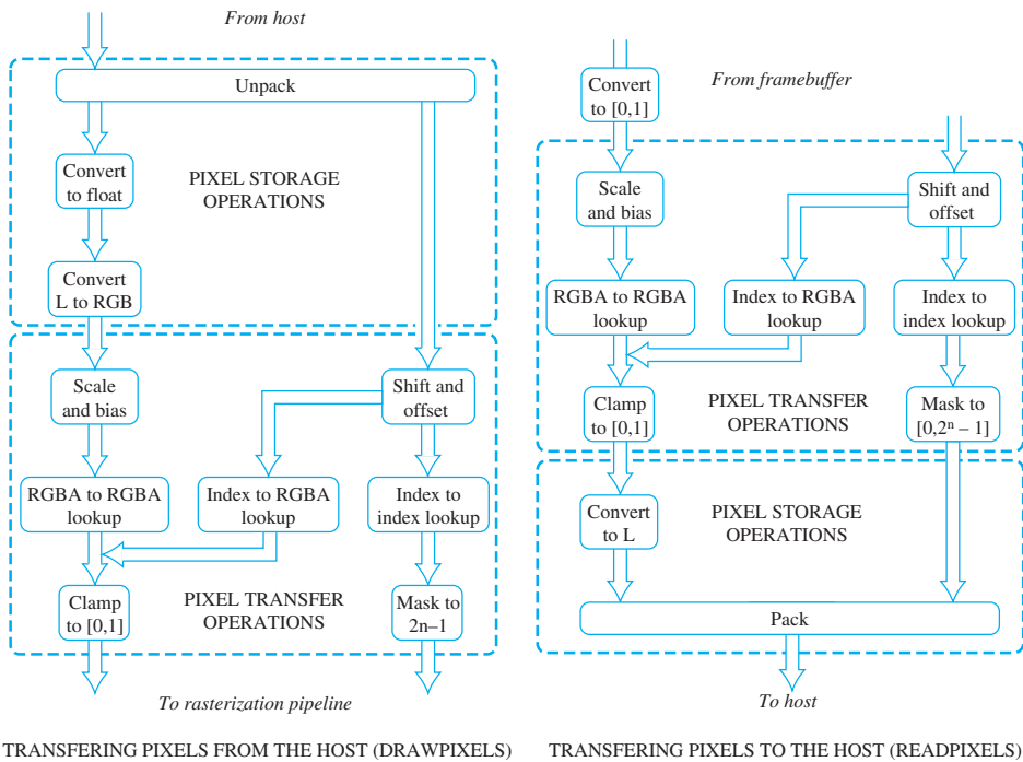
Figure 4.6 Basic pixel pipeline.
