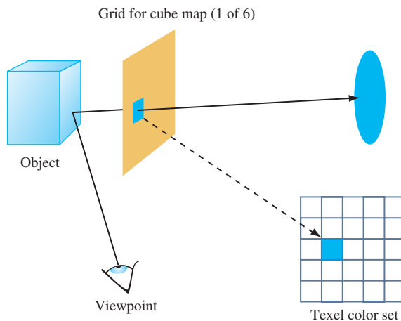
Figure 17.21 Creating environment maps using ray casting.
