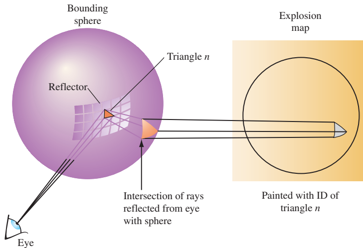
Figure 17.9 Mapping reflection vectors into explosion map coordinates.
