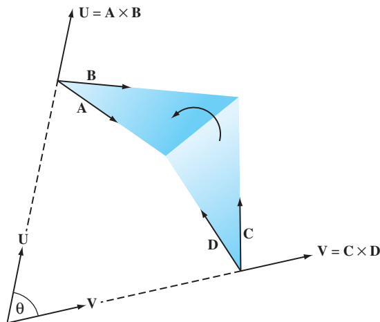
Figure 1.1 Quadrilateral decomposition.
