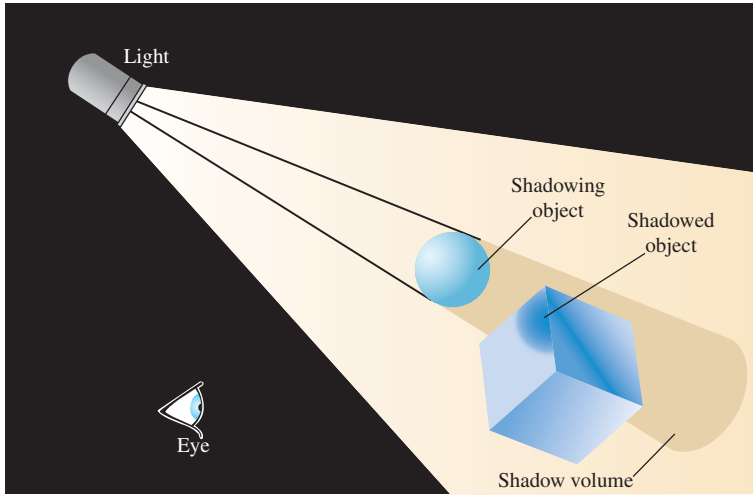
Figure 17.27 Shadow volume.
