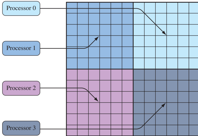
Figure 8.3 Screen tiling.
