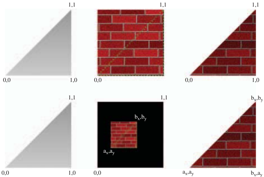
Figure 14.4 Texture mosaicing.
