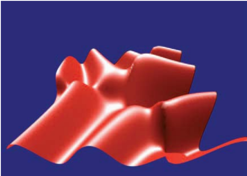
Figure 20.9 Rubber sheeting.
