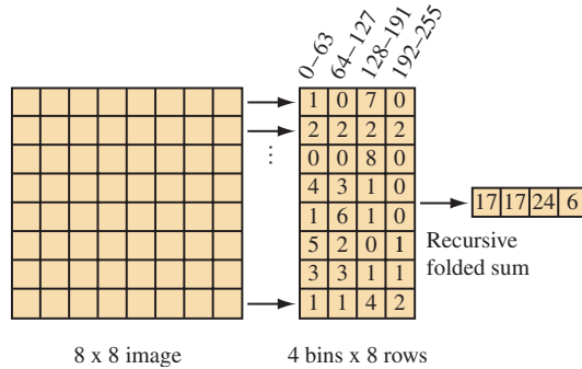
Figure 12.4 Multi-row histogram and folded sum.
