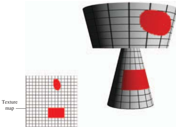
Figure 19.15 Painting on a 3D object.
