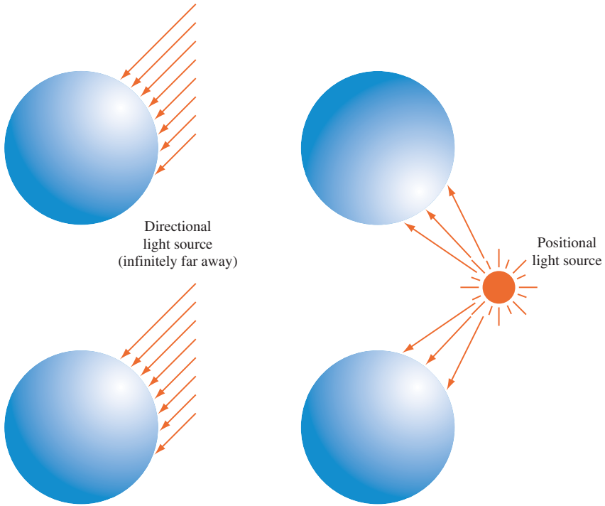
Figure 3.7 Directional and positional light sources.
