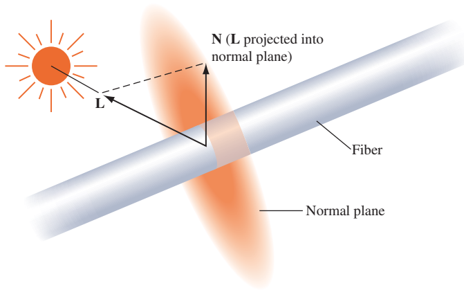
Figure 15.8 Projecting light vector to maximize lighting contribution.
