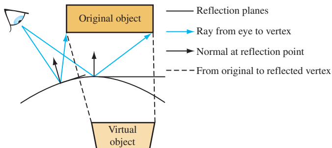
Figure 17.5 Normals and reflection vectors in curved reflectors.
