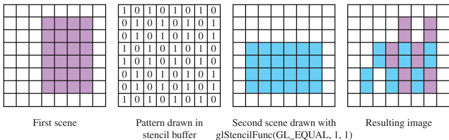
Figure 11.1 Using stencil to dissolve between images.
