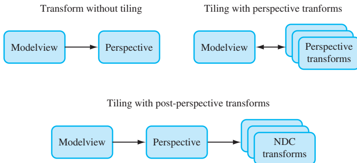
Figure 13.3 Image tiling transforms.
