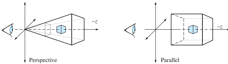
Figure 2.8 Perspective and parallel projections.
