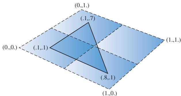
Figure 14.5 Texture tiling.
