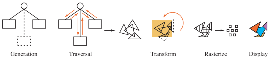
Figure 21.2 The stages of a graphics update.
