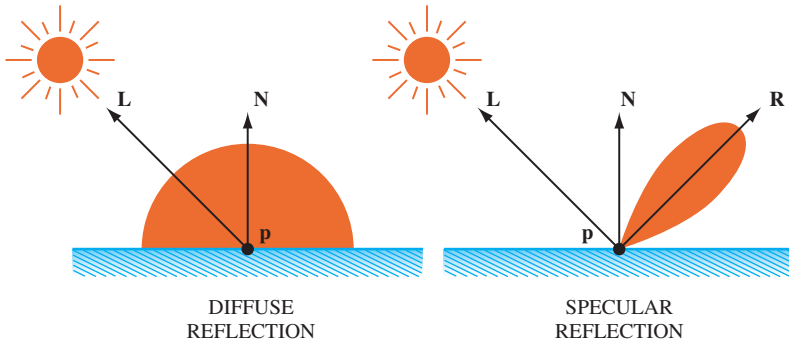
Figure 3.6 Diffuse and specular reflection patterns.
