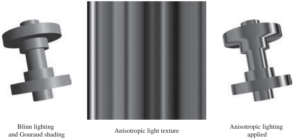
Figure 19.4 Simulation of anisotropic lighting.
