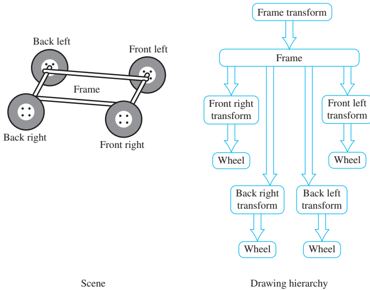
Figure 16.1 Instancing of four wheels.
