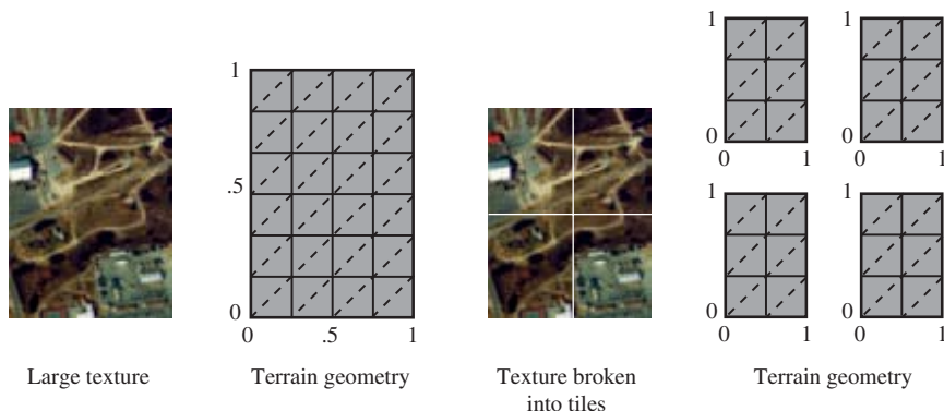
Figure 14.7 Modeling a large texture as a grid of tiles.
