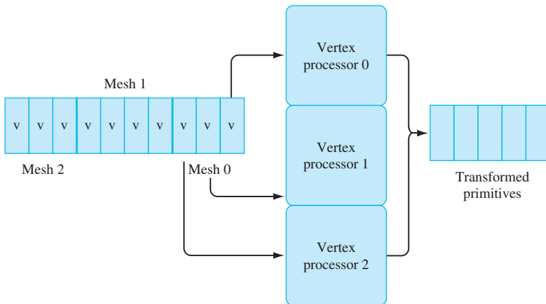
Figure 8.2 SIMD vertex processing.
