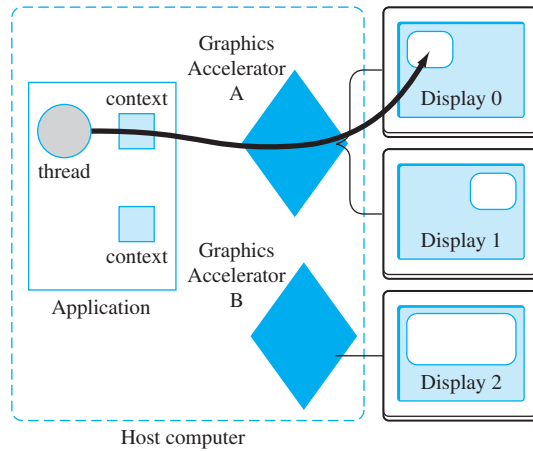
Figure 7.2 Three-display system using two accelerators.
