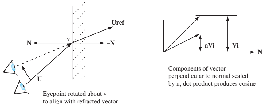
Figure 17.17 Changing viewpoint angle to simulate refraction.
