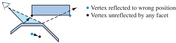
Figure 17.7 Approximating a curved reflector as triangle facets.
