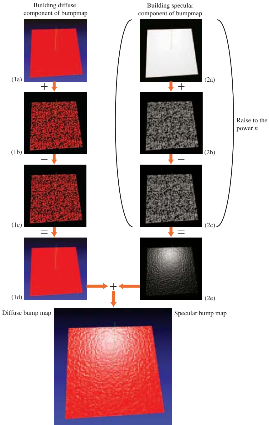
Figure 15.13 Bump mapping: shift and subtract image.
