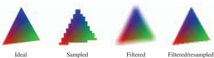
Figure 4.1 Example of image reconstruction.
