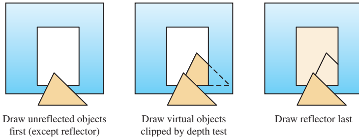
Figure 17.3 Masking reflections with depth buffering.
