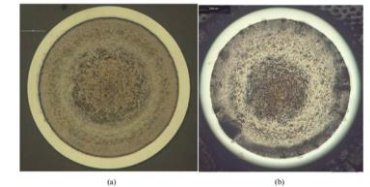
Figure 69. Metallography of Pu-12Am-40Zr irradiated to approximately 20% burnup in: a) Phenix fast reactor (FUTURIX-FTA DOE2), and b) cadmium-filtered position in ATR (AFC-ID R4).
