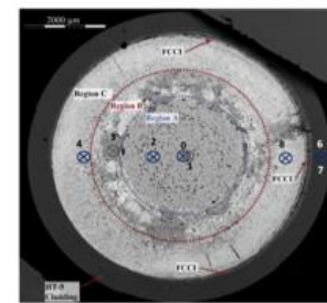
(a) SEM image of a polished section of the irradiated U-10 wt.% Zr fuel pin. The TCM measurement locations on the profile of the pin are marked along with the measurement number.
