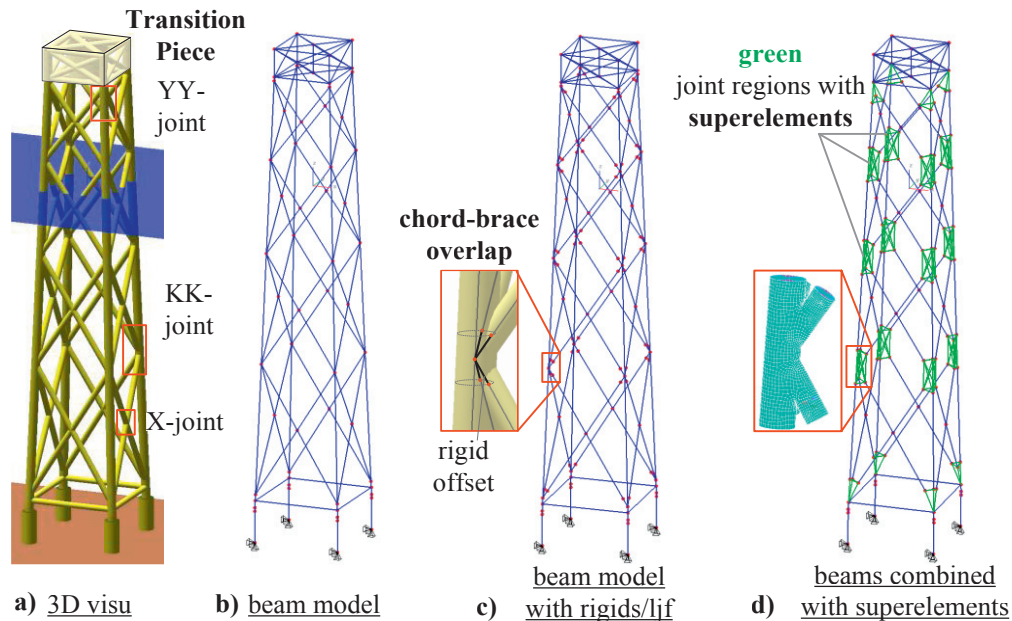
Figure 1: a) 3D Visualization of the OC4 jacket [11] and simulation models with different levels of detail from b) a simple to d) a sophisticated approach taking local joint flexibilities (liff) into account
