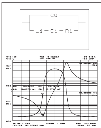
Equivalent Component Analysis (Resonator)
