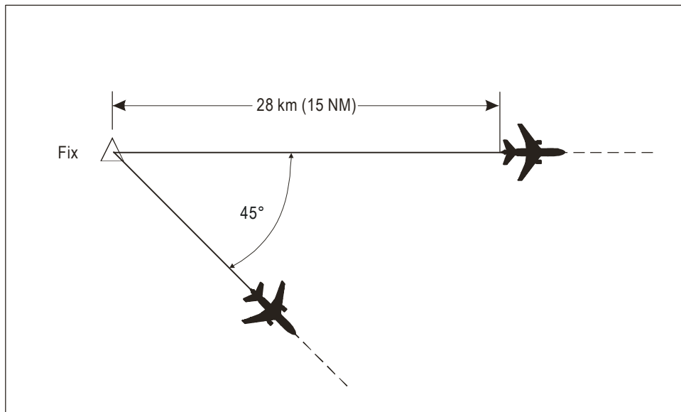
Figure 5-4. Separation using dead reckoning (see 5.4.1.2.1.2 c))
