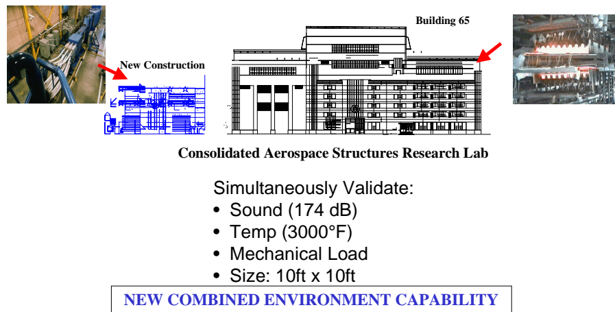
Fig. 7 AFRL's new Consolidated Aerospace Structures Research Laboratory will simulate combined extreme acoustic, thermal and mechanical loads.
