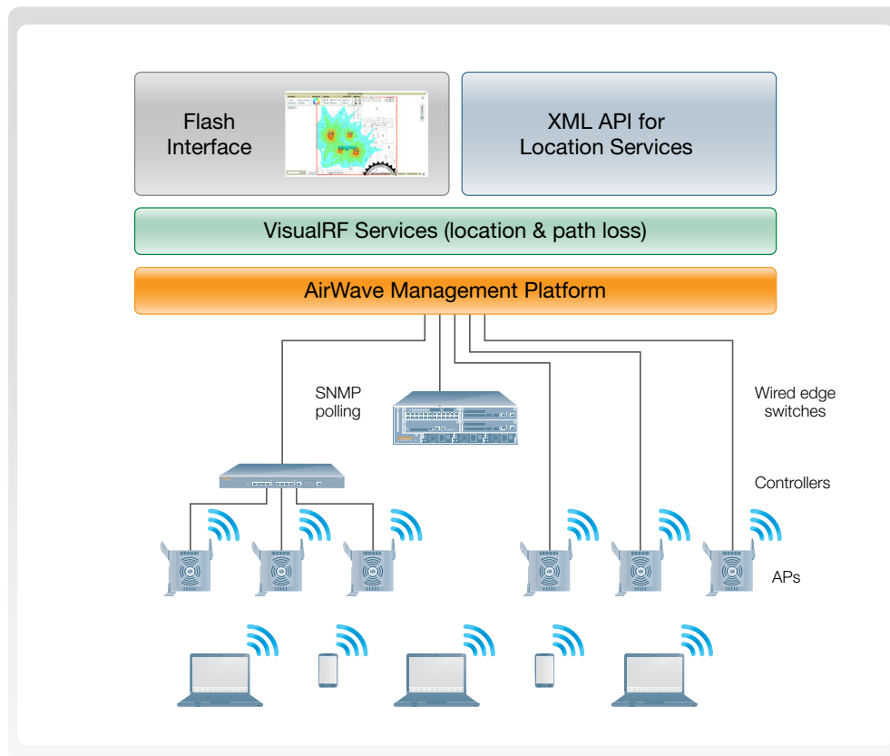
Figure 4. The AirWave Management Platform, a core component of the AirWave Management Suite, provides efficient, centralized management of your wireless infrastructure and visibility across the wired edge of your network.
