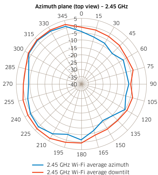
Figures. OmniAccess AP1311 antenna pattern plots
