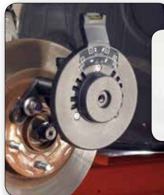
Kit 20-2577-1 includes two adaptors
