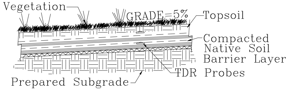
Figure 2. Prescriptive RCRA Subtitle D landfill cover design.
