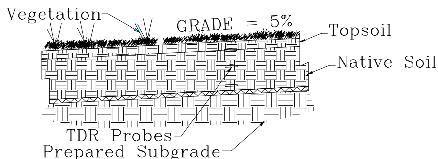
Figure 13. Evapotranspiration cover design.
