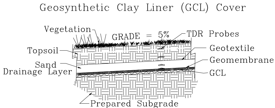
Figure 7. GCL cover design.
