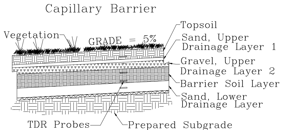
Figure 9. Capillary barrier cover design.
