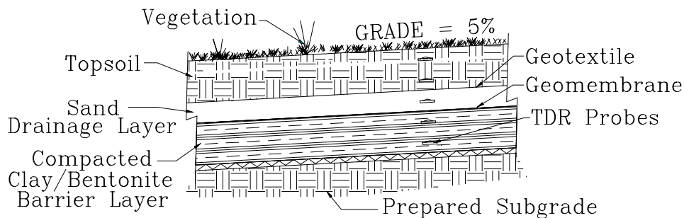
Figure 3. Prescriptive RCRA Subtitle C landfill cover design.
