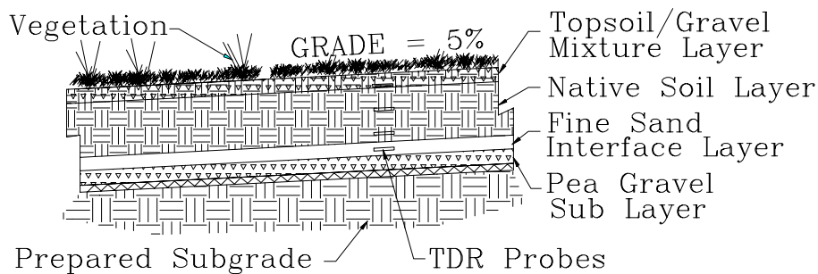
Figure 11. Anisotropic barrier cover design.
