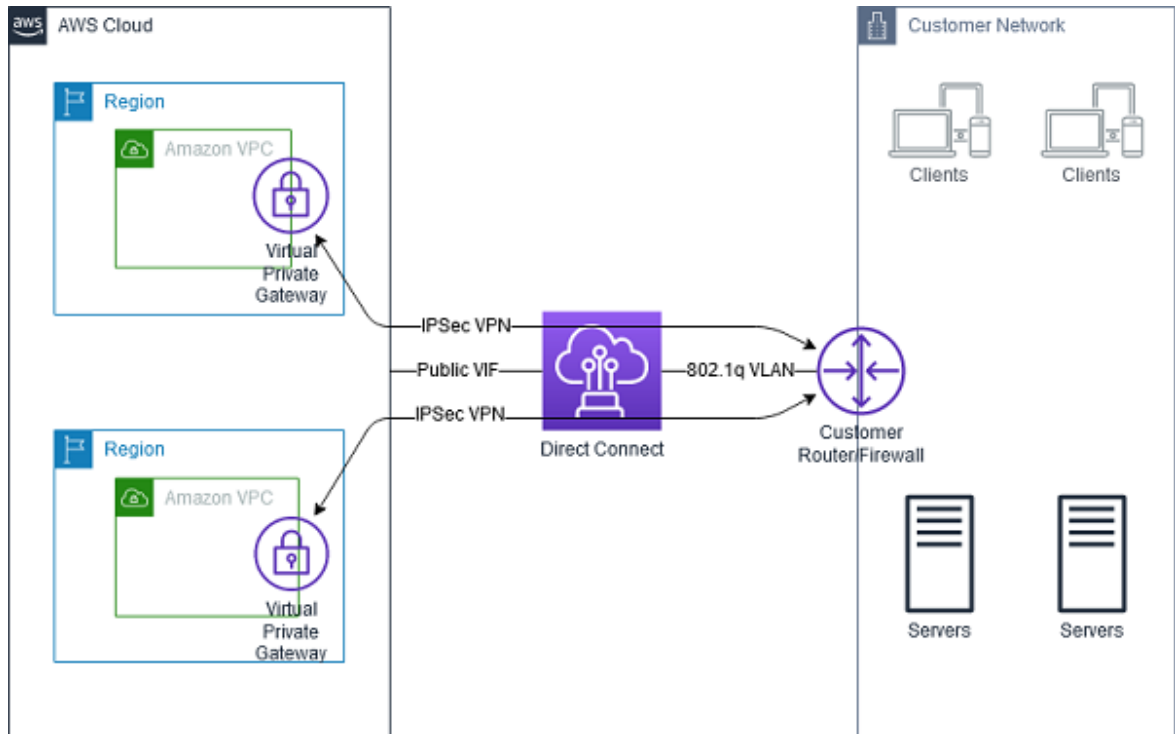
Figure 9 - AWS Direct Connect and VPN
