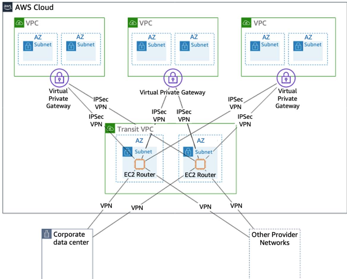
Figure 22 - Transit VPC
