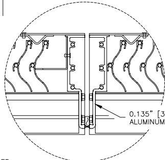
(F) RECESSED VERTICAL MULLION DETAIL OPTIONAL MULLION CONFIGURATION
