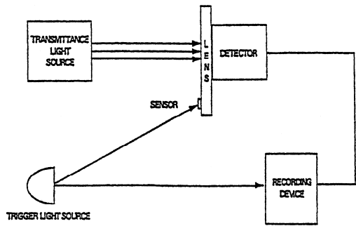
Figure E2 Switching Index Tightness Test Apparatus
