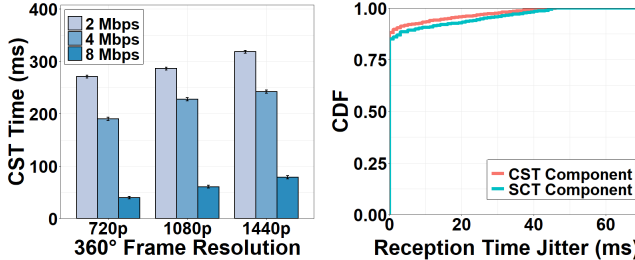
Figure 11: CST time versus upload bandwidth.
