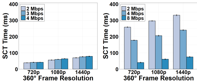
Figure 15: SCT time under different bitrates.
