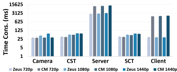
Figure 19: Comparison of component time between Zeus and a commercial system (denoted by CM).
