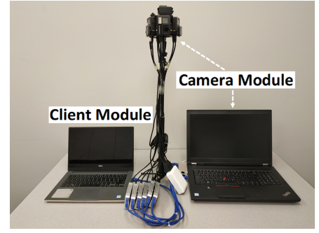
Figure 2: The Zeus prototype.
