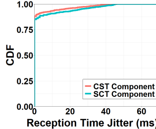
Figure 12: Jitter of packet reception time.
