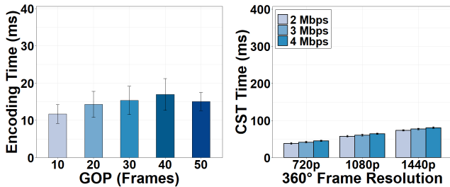
Figure 9: Encoding time of a 720p frame versus GOP.
