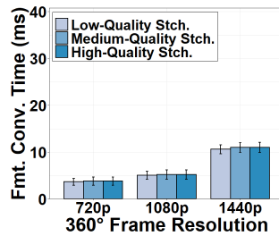
Figure 7: Format conversion time vs. stitching options.
