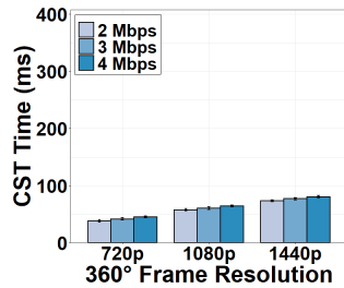
Figure 10: CST time under different bitrates.
