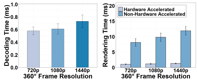
Figure 17: Decoding time versus 360° frame resolutions.
