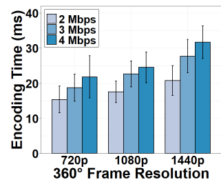
Figure 8: Encoding time under different bitrates.
