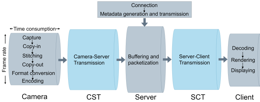
Figure 1: The architecture of live 360° video streaming and the tasks of the 5 system components. The top rectangle shows one-time tasks whereas the 5 bottom pipes show the pipeline tasks that must be passed through for every frame.
