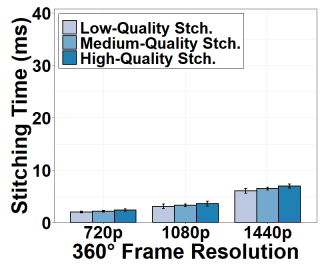
Figure 6: Frame stitching time vs. stitching options.
