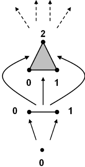
Figure 8: A partial illustration of the category \widehat{\Delta}
