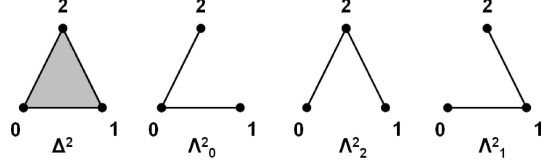
Figure 22: The three horns on |\Delta^2|
