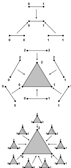
Figure 11: The first picture represents all of the 1-simplices in |\Delta^1| , including the degenerate ones that are taken to individual vertices. The second picture represents all the 1-simplices in |\Delta^2| , and the last picture represents all of the degenerate 2-simplices in |\Delta^2| .
