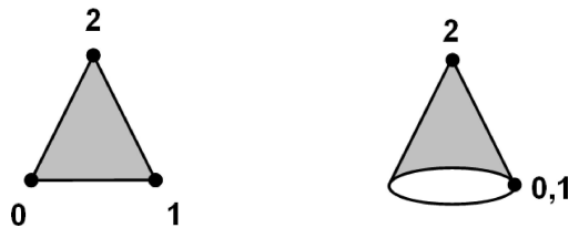
Figure 6: Gluing |\Delta^2| into a cone
