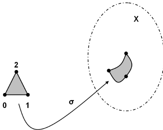
Figure 12: A singular simplex
