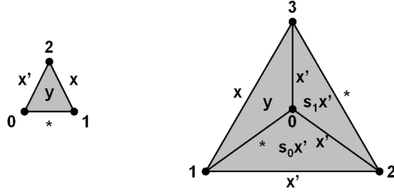
Figure 27: Shifting indices in the homotopy relation. Here * represents d_2s_0x = d_2s_0x' , which is a degenerate 1-simplex, both vertices being the first vertex of x , which is also the first vertex of x' .
