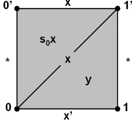
Figure 28: We label the vertices with the “prism notation” of Example 5.5. The bottom simplex y is a homotopy of the simplices x and x' . Adjoining the degenerate simplex s_0x shows how to obtain a model prism for the homotopy from x to x' as inclusion maps.
