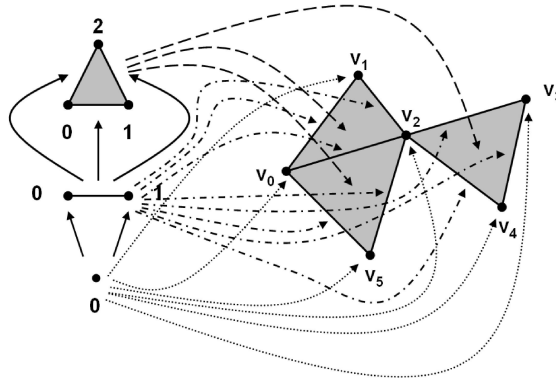
Figure 9: A Delta complex as the functorial image of \widehat{\Delta}
