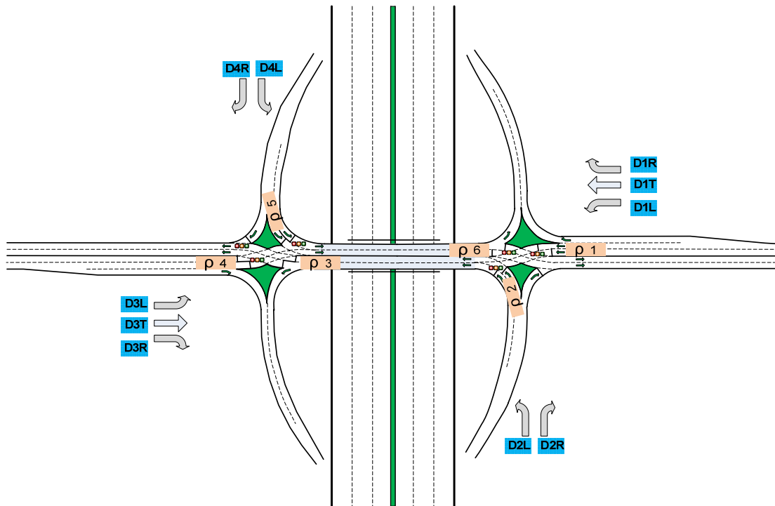
Figure 3-19: Spatial distribution of all factors associated with the total delay at a DDI
