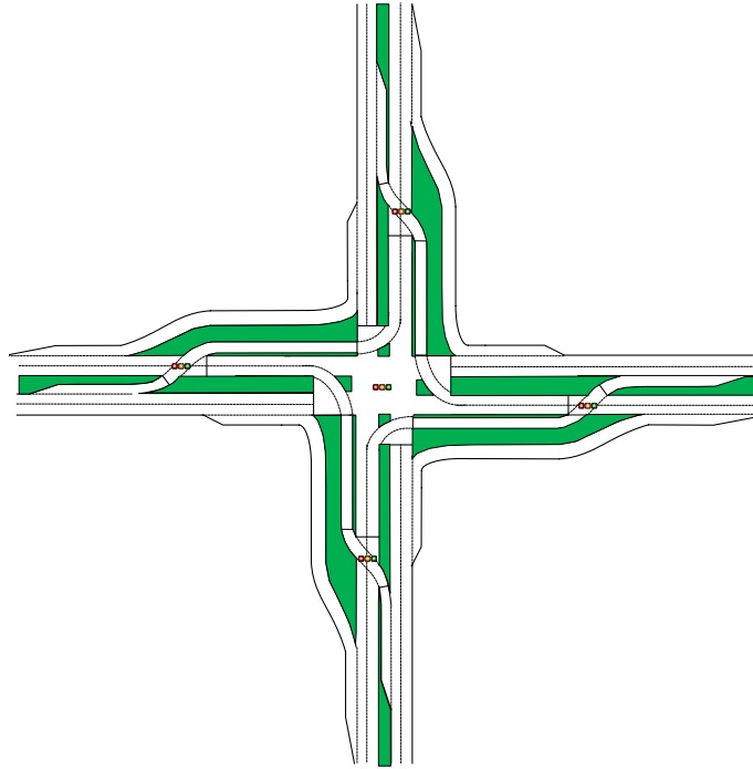
Figure 2-1: Graphical illustration of a full CFI design
