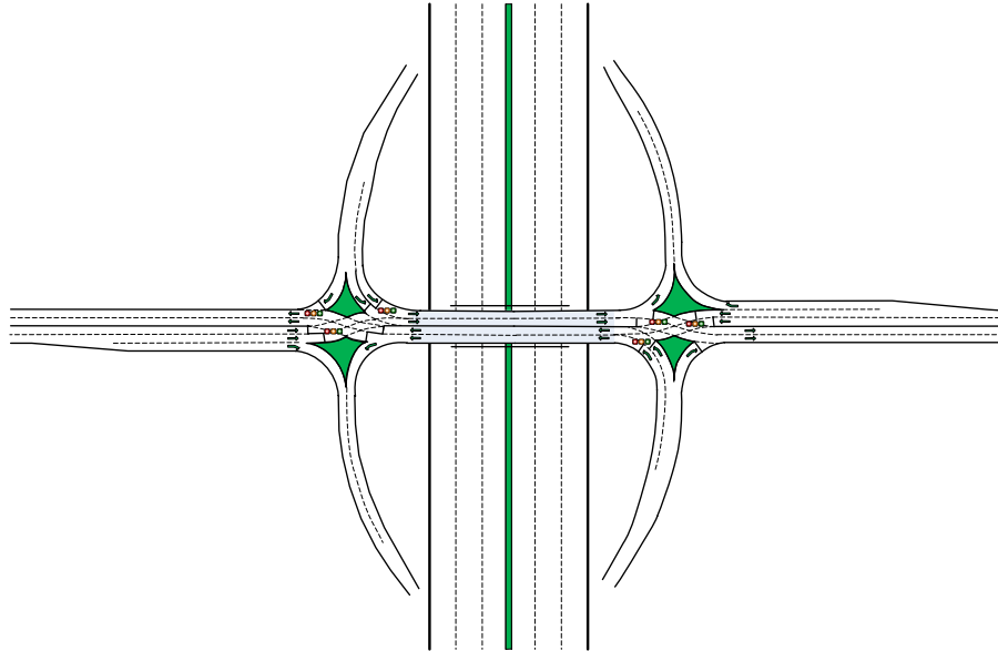
Figure 3-1: Bird's eye view of a typical DDI design
