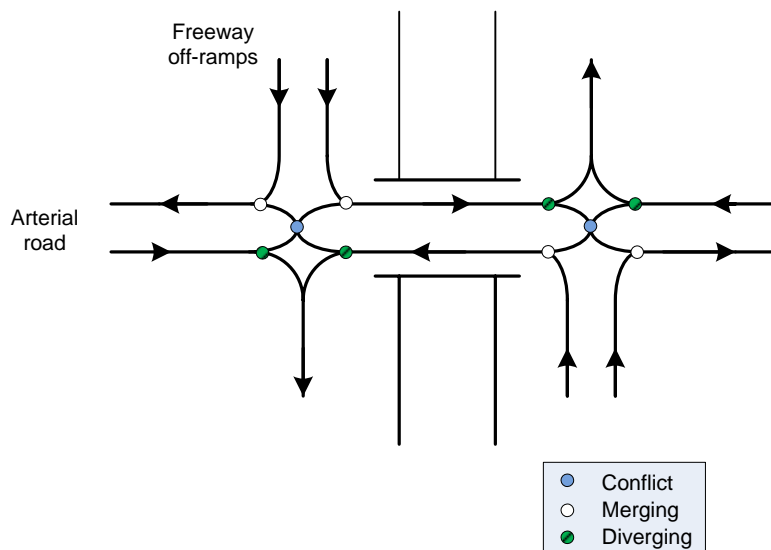
Figure 3-8: Conflict points of a DDI
