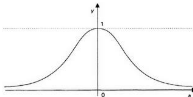
Figure 10.13 One-dimensional Gaussian.
