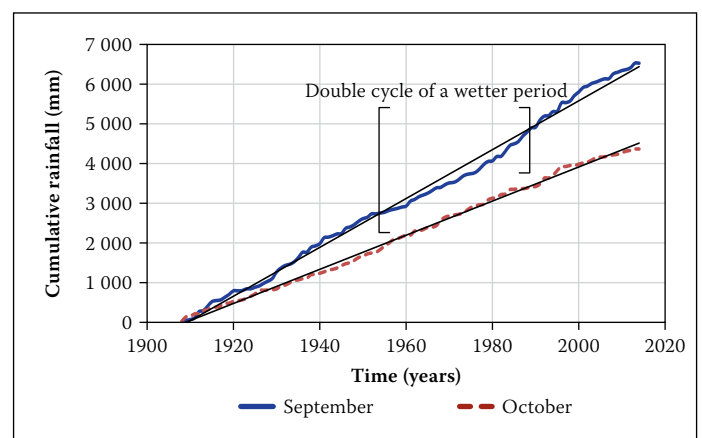
Figure 10(b): Cumulative total monthly rainfall distribution for September and October over the full record length (South African Astronomical Observatory Rainfall Station)
