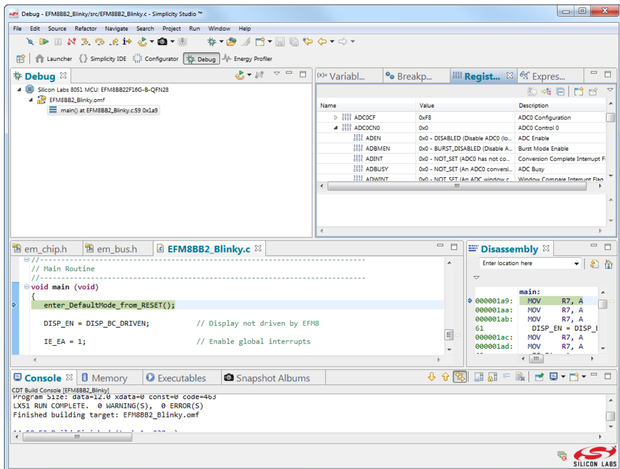
Figure 4.1. Debugger
