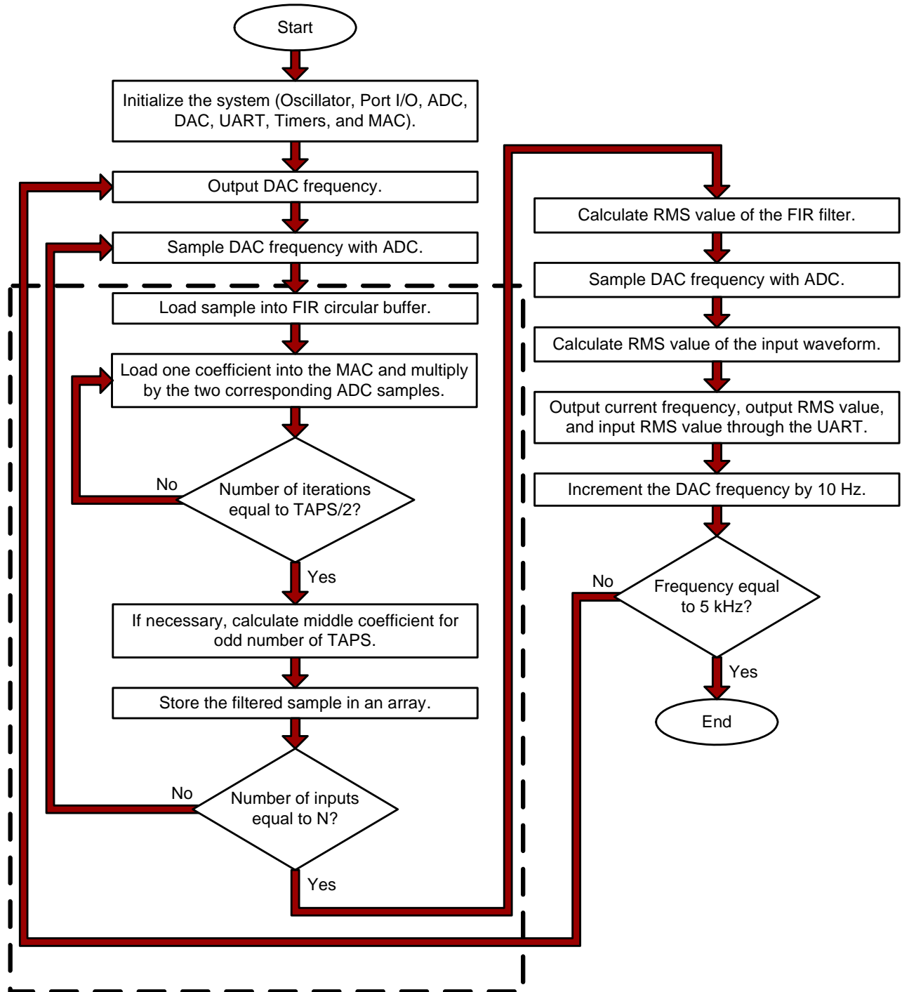
Figure 1. FIR Filter Firmware Flow Diagram
