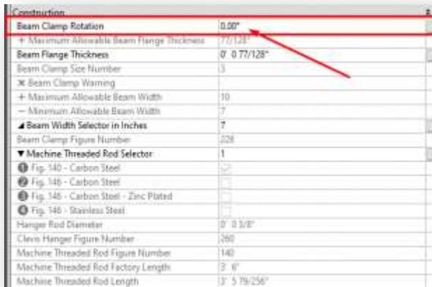
Example 18: Default rotation angle of 0 in Revit.
