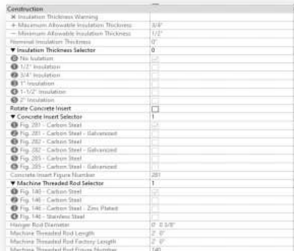
Example 13: More Construction Group parameters.
