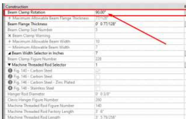
Example 19: Beam Clamp with 90-degree rotation angle in Revit.
