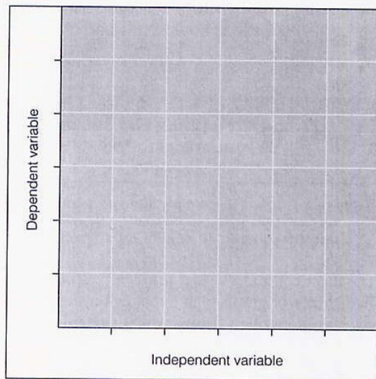
Figure 2.5. Graph construction.
