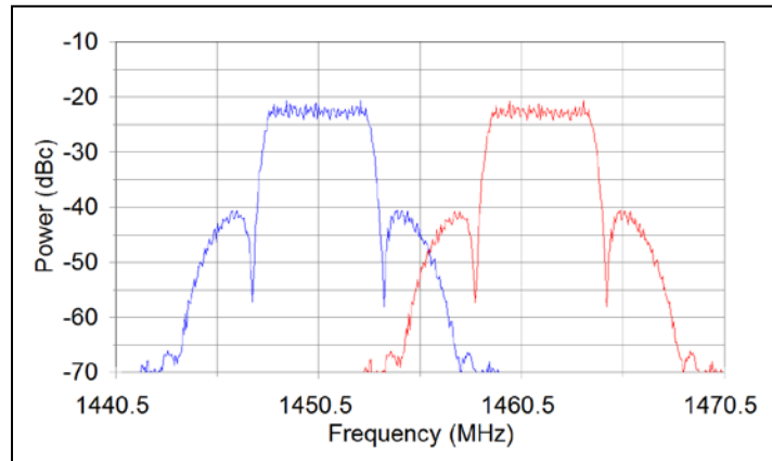
Figure A-2. 5 Mbps PCM/FM Signals with 11 MHz Center Frequency Separation
