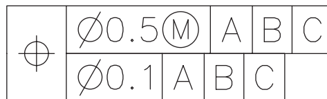
Figure A1-12. Specifying information for a double feature control frame in the Geometric Tolerance dialog box.
