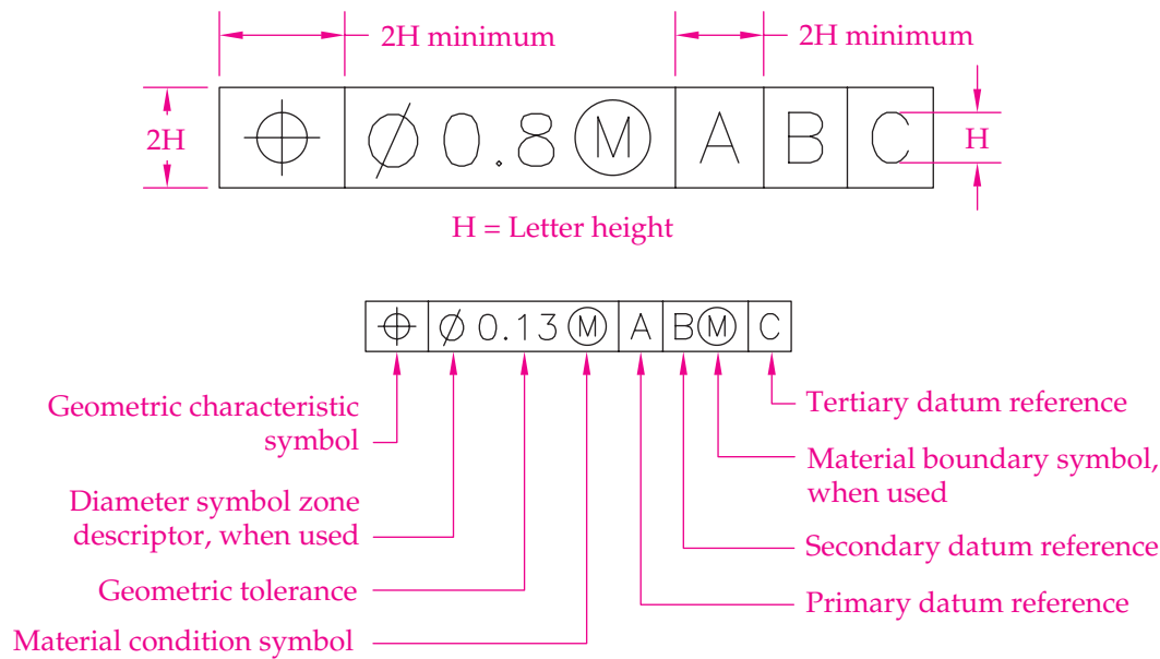
Figure A1-5. The order of elements in a feature control frame.
