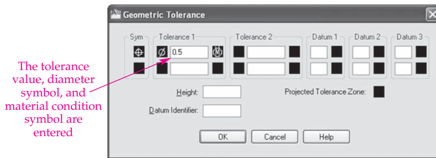
Figure A1-4. The Geometric Tolerance dialog box with a diameter symbol, geometric tolerance value, and maximum material condition (MMC) symbol added to the Tolerance 1 area.
