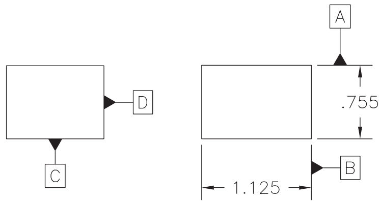
Figure A1-15. Examples of datum feature symbols created using a combination of the TOLERANCE and MLEADER or QLEADER tools.
