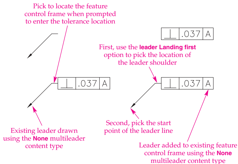
Figure A1-9. Use the MLEADER tool to create a leader before drawing the feature control frame using the TOLERANCE tool, or add the leader to an existing feature control frame.
