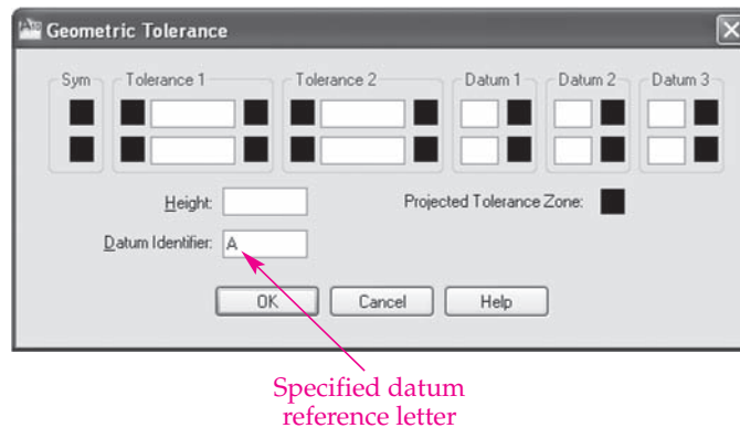
Figure A1-14. Using the Geometric Tolerance dialog box to enter a datum-identifying reference letter. The letter creates the datum identifier.
