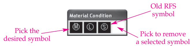
Figure A1-3. The Material Condition dialog box. Notice that the symbol for regardless of feature size (RFS) is available. ASME Y14.5-2009 does not use this symbol, but you may need it when editing older drawings.
