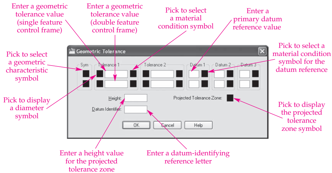
Figure A1-1. You can use the Geometric Tolerance dialog box to draw geometric dimensioning and tolerancing (GD&T) symbols and feature control frames.
