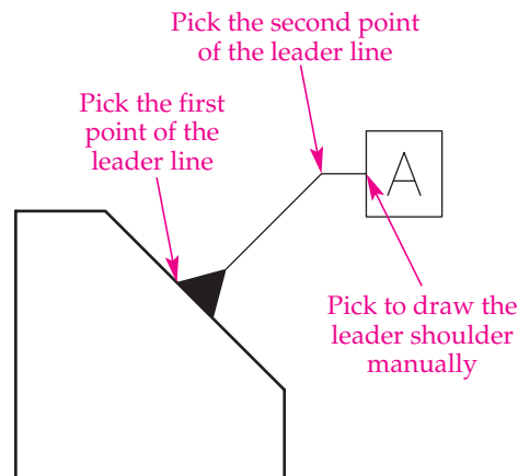
Figure A1-17. Use the Tolerance annotation option of the QLEADER tool to add a datum feature symbol to an angled surface.
