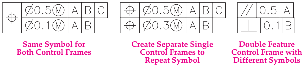
Figure A1-13. If you enter the same geometric characteristic symbol in both Sym boxes of the Geometric Tolerance dialog box, only one symbol appears in the first compartment of the feature control frame. Create two separate feature control frames to display the same symbol in both frames. If you use two different symbols, they appear in separate compartments.
