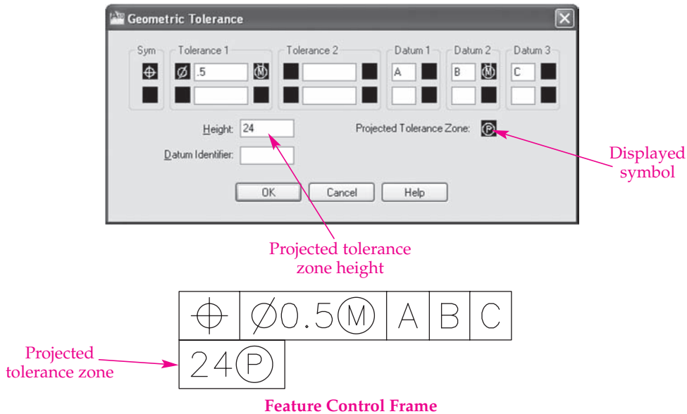
Figure A1-10. To add projected tolerance zone specifications in accordance with ASME Y14.5M-1982, enter the projected tolerance zone height and symbol in the Geometric Tolerance dialog box.
