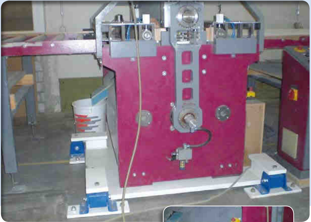
Resilient suspension of punching press
