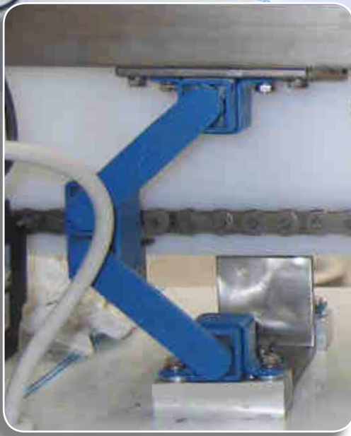
Suspensions of chocolate compactors
