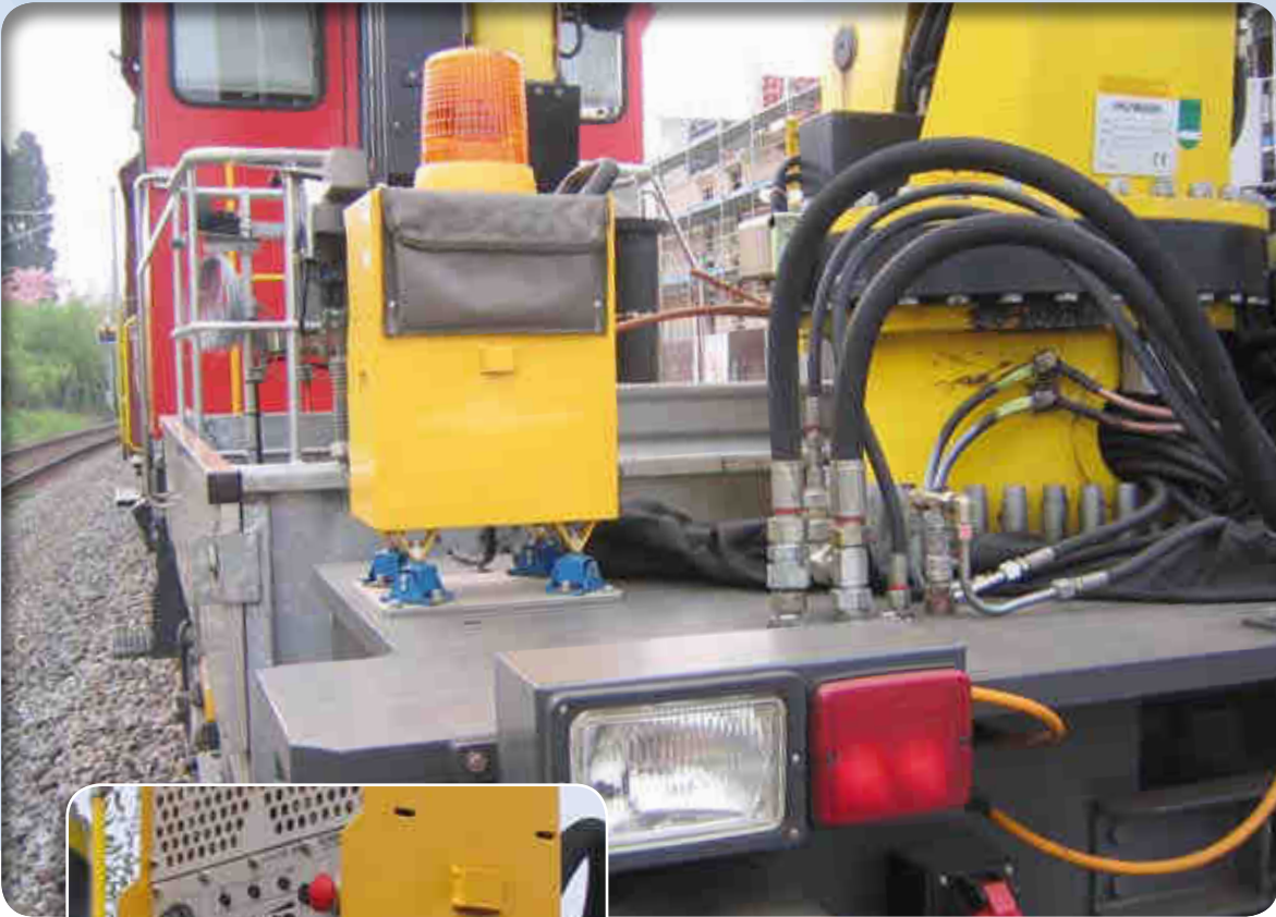
▲ Protective suspension of electronic device on track car
