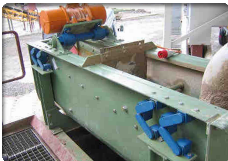
Suspensions of gravel washing trough
