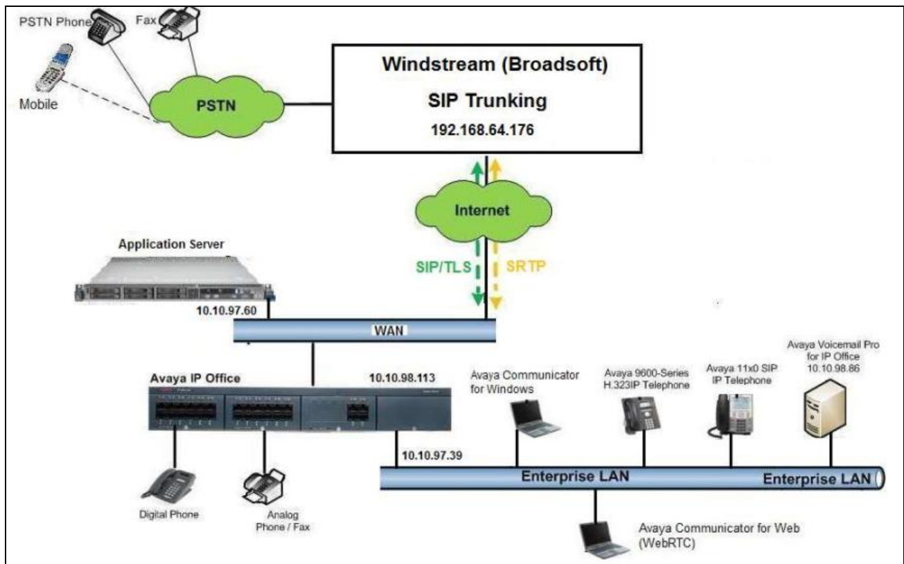
Figure 1: Test Configuration for Avaya IP Office with Windstream SIP Trunking Service
