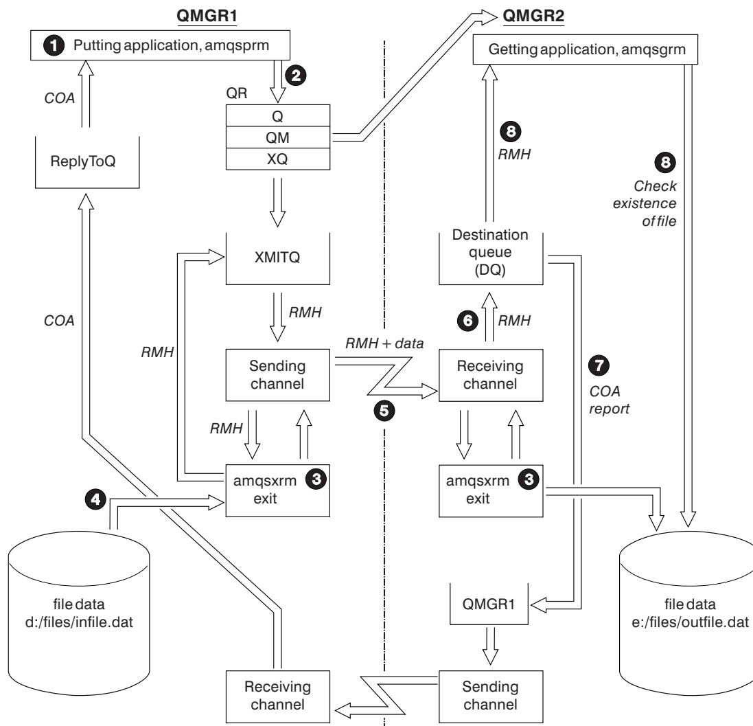
Figure 35. Running the Reference Message samples
