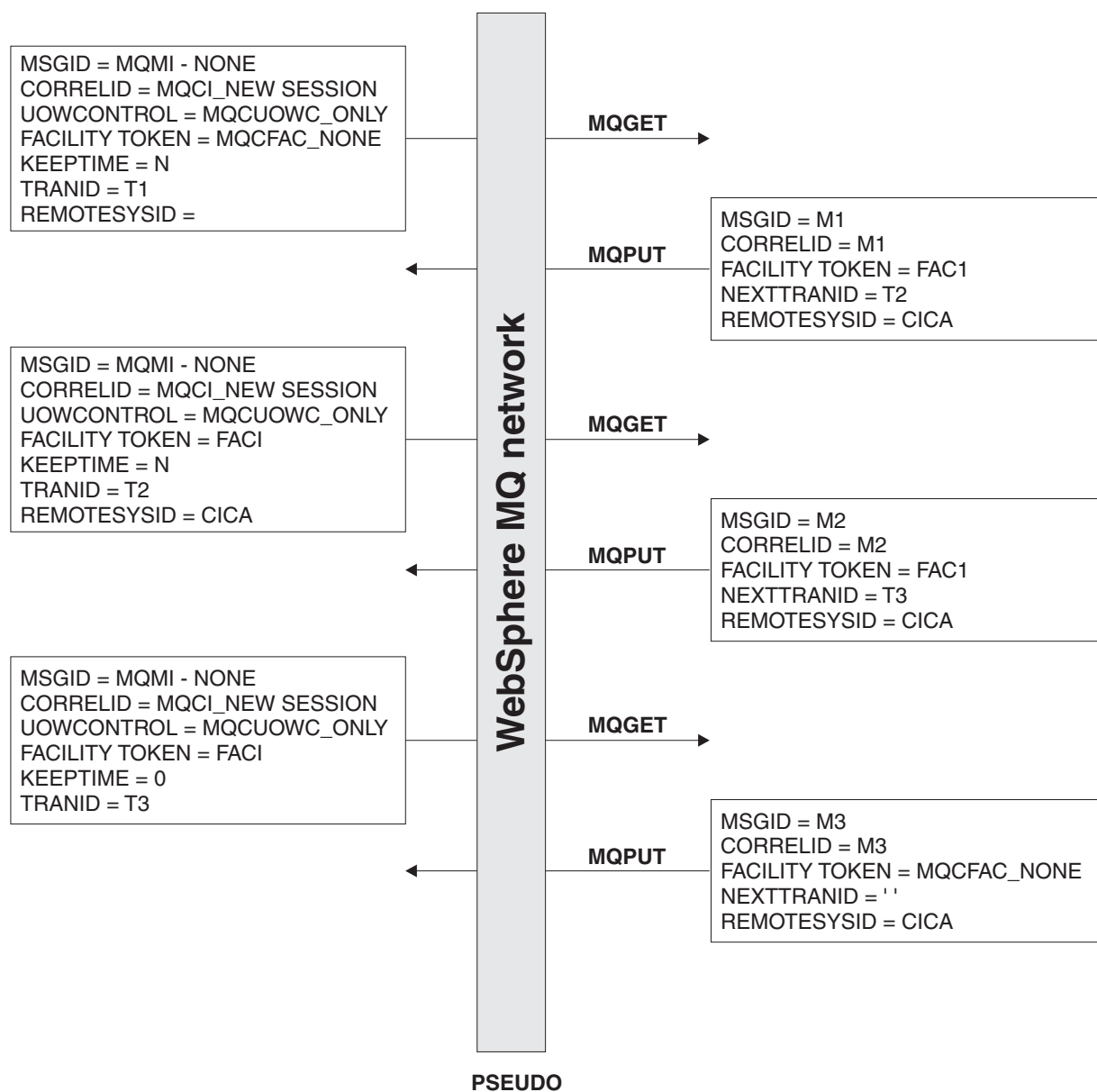
Figure 17. Setting of key fields: WebSphere MQ - pseudo-conversational 3270 transaction viewed from the perspective of the bridge prior to CICS TS 2.2
