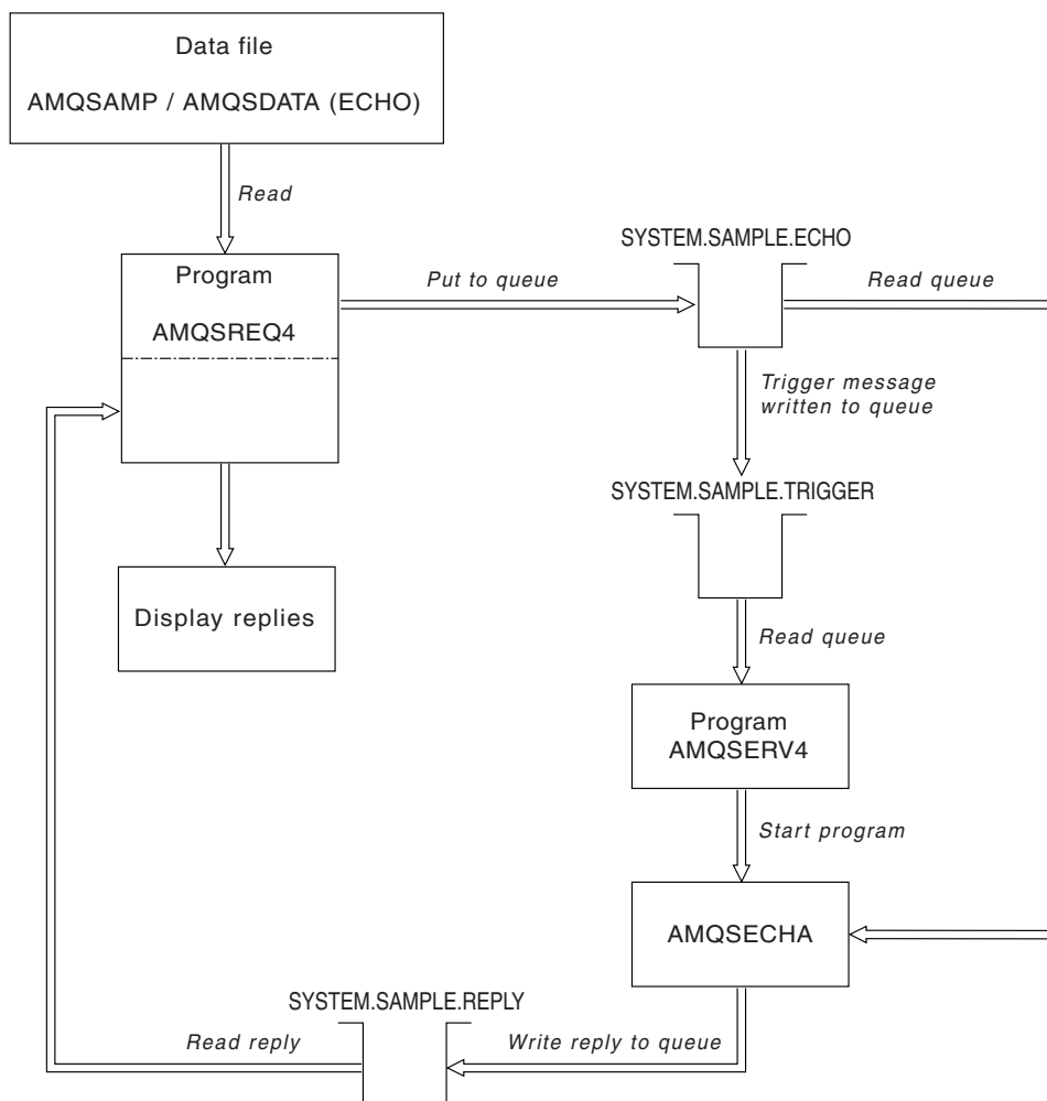
Figure 37. Sample i5/OS Client/Server (Echo) program flowchart
