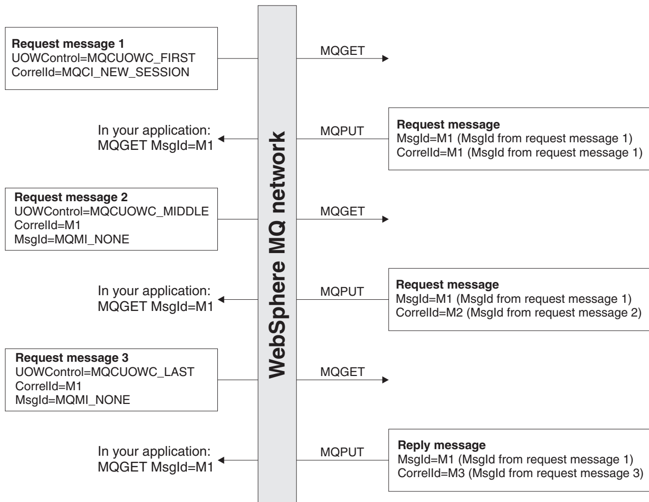
Figure 16. Setting of key fields for many CICS user programs in a unit of work viewed from the perspective of the bridge
