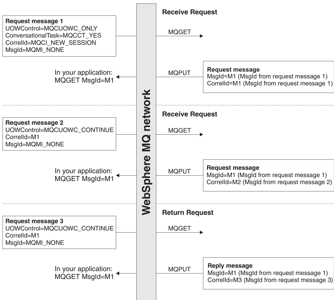
Figure 18. Setting of key fields: WebSphere MQ - conversational 3270 transaction viewed from the perspective of the bridge
