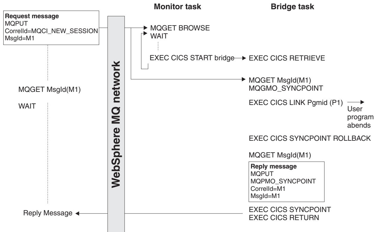
Figure 19. User program abends (only program in the unit of work)
