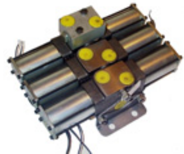
△ Boom Hydraulic Directional Control Valve Assembly (3 Spool) for Older B-Series A110496 (12 Volt) A110501 (24 Volt) NOTE: See parts bulletin AQP-B-128 for components.
