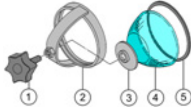
△ Sight Eye Assembly A153007
