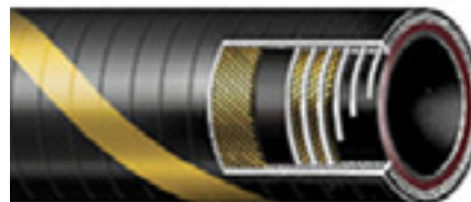
△ Water Supply Hose A176470 (3" I.D. Water Supply Hose) A176480 (4" I.D. Water Supply Hose) Hose sold per foot Compatible with a variety of models
