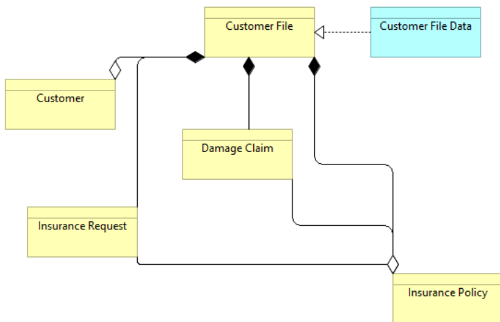
Manhattan Router
