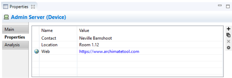
User Properties
