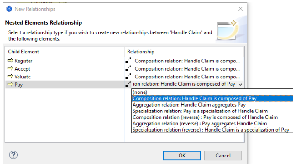
Dialog for creating more than one relationship
