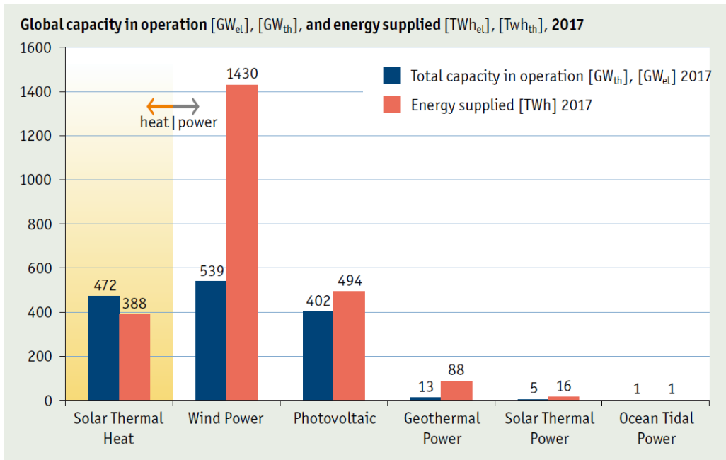
Figure 118: Global installed capacity and energy yield of solar thermal compared to other major renewable energy technologies. Note that solar thermal is in GW th /TWh th while the other technologies are in GWe/TWhe. Reproduced from (Weiss & Spörk-Dür, 2018).
