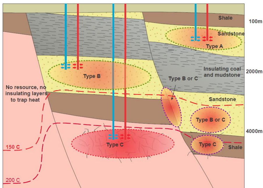
Figure 90: Geothermal resources and the three main types of use. Reproduced from CSIRO, (Huddlestone-Holmes, 2014).
