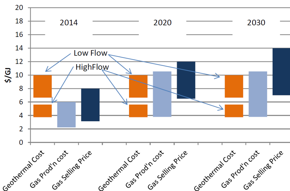
Figure 96: Comparison of geothermal energy cost, gas production cost and gas selling price at Moomba. (Reproduced from (Evans & Peck, 2014)).
