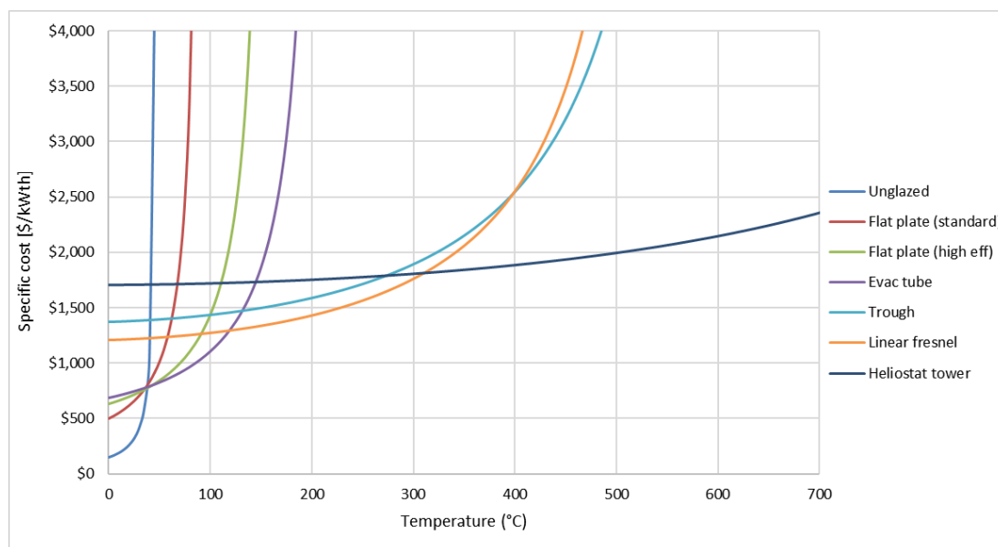
Figure 122: Indicative capital costs with temperature.
