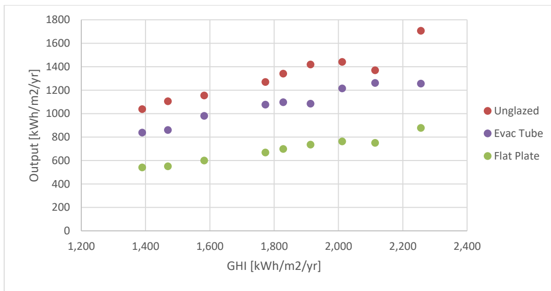
Figure 127: Collector output vs GHI by location.
