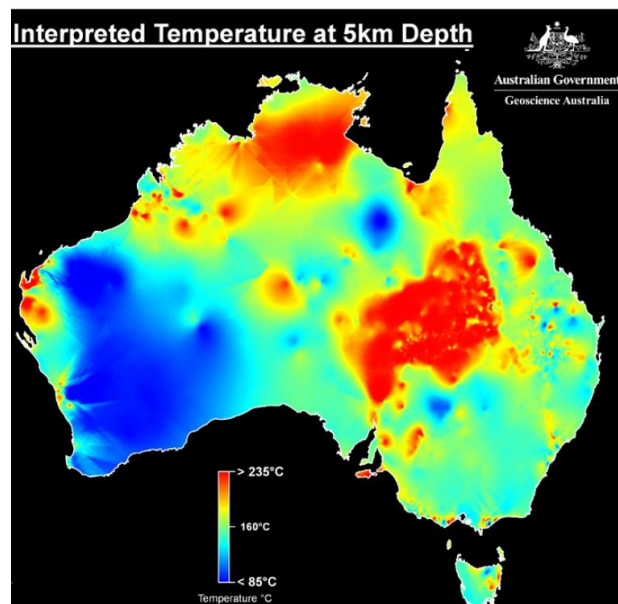
Figure 92: Interpreted crustal temperature at 5 km depth. Reproduced from Geoscience Australia.
