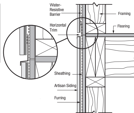
Figure 13 Bridging Floors
