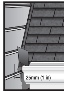
Figure 12 Valley/Shingle Extension
