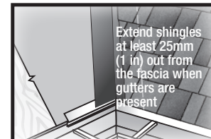
Figure 12 Valley/Shingle Extension
