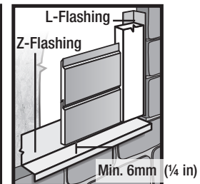
Figure 9 Mortar/Masonry
