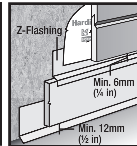
Figure 8 Sheltered Areas
