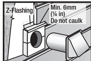
Figure 11 Block Penetration
