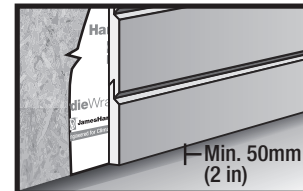
Figure 9 Mortar/Masonry
